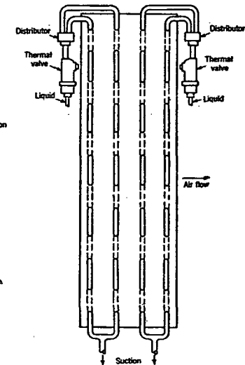
FIG. 7. ARRANGEMENT FOR DEPTH CONTROL
