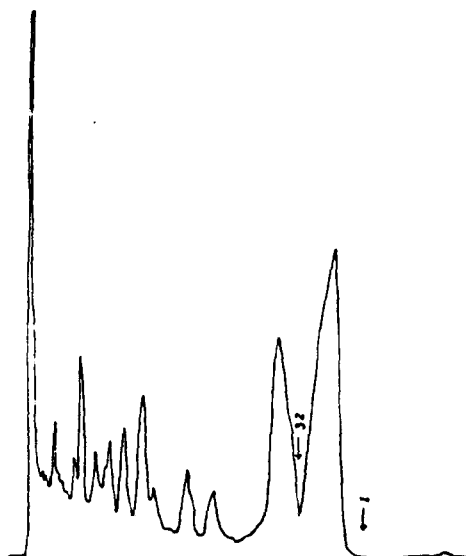
Fig. 7.—Gas chromatogram of extract from sample X-74 showing the number of components in the light fraction (up to 16 minutes) and the two components in the heavy fraction (plasticizers). Note: Same time scale as in Fig. 6.
