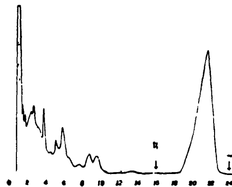
Fig. 6.—Gas chromatogram of extract from sample X-37 showing the number of components in the light fraction (up to 16 minutes) and the one component in the heavy fraction (plasticizer).
