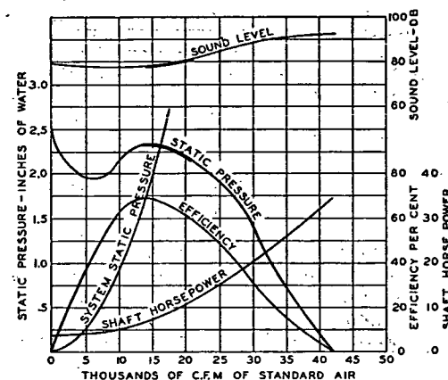
FIG. 1. SOUND LEVEL CHARACTERISTICS OF TYPICAL CENTRIFUGAL, MULTI-BLADE VENTILATING FAN.
