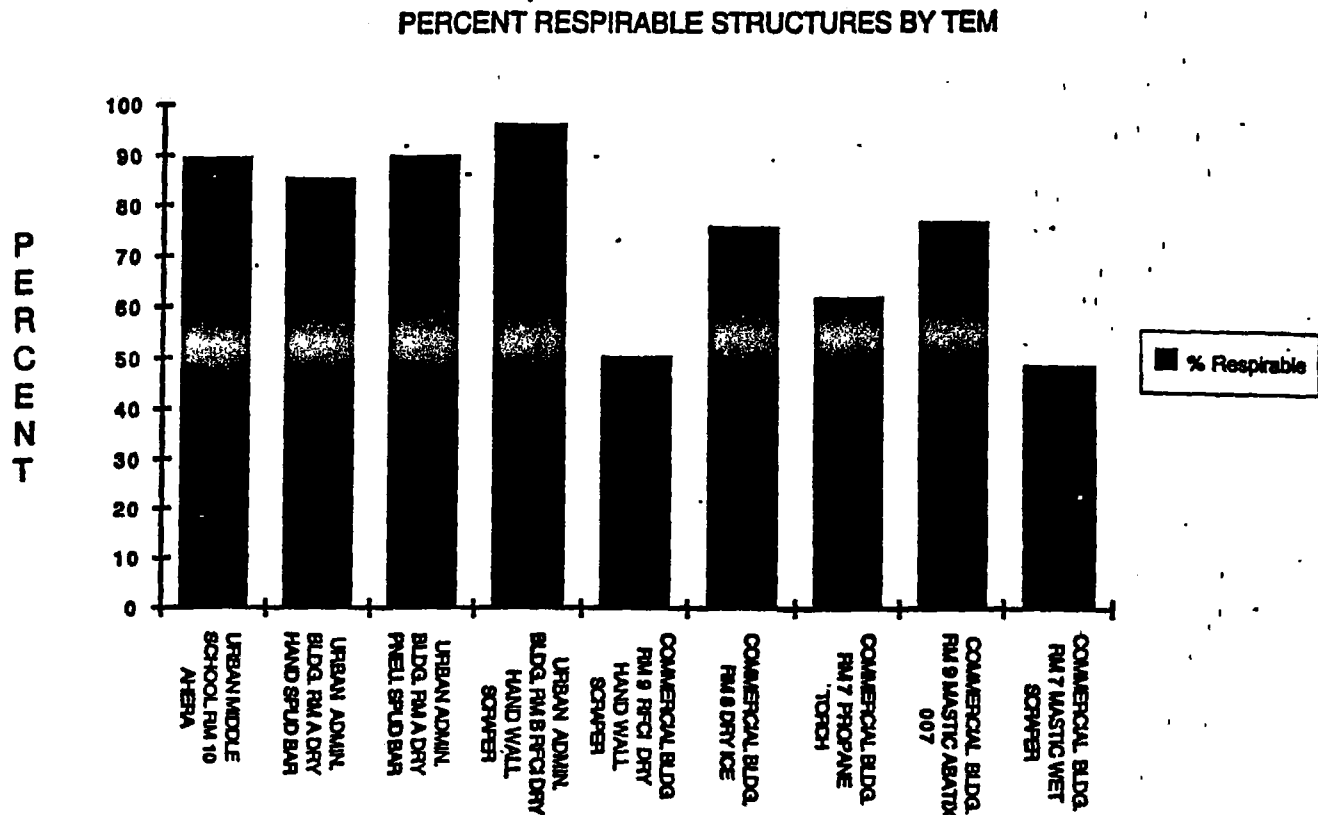
FIGURE 9. Percent respirable asbestos structures by ATEM.
