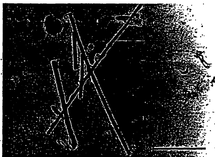
FIGURE 6. ATEM micrograph of chrysotile fibers seen only by electron microscopy. Source was the East Texas commercial building Abatix 007 mastic procedure. Bar = 1 \mu\text{m} .
