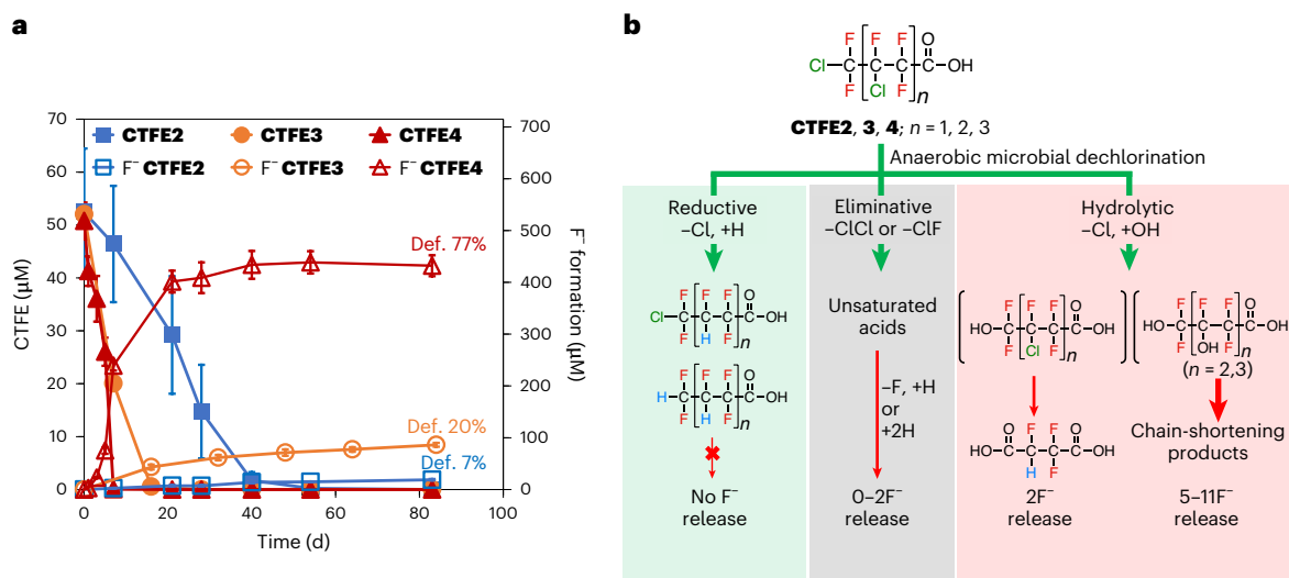
Fig. 1 | Biotransformation and defluorination pathways of CTFE oligomer carboxylic acids by the anaerobic microbial community. a , Parent compound decay and F⁻ formation over 84 days. The data are presented as mean values. The error bars represent the s.d. from n = 3 replicate experiments. Def., defluorination. b , The proposed general biotransformation pathways. Green arrows represent dechlorinating reactions. Red arrows represent defluorinating reactions. The thickness of the red arrows represents the number of F⁻ ions released. The green-shaded panel shows the non-defluorinating
