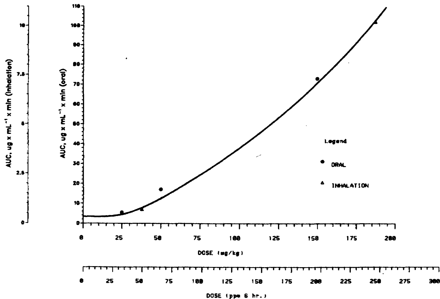
Figure 9-13. Relationship in Sprague-Dawley rats between the area under the blood EDC concentration-time curve (AUC) and the gavage dose of EDC in corn oil (mg/kg) or inhaled doses of EDC (ppm for 6 hours).
