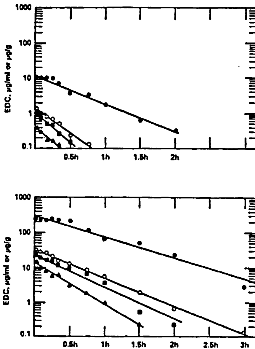
Figure 9-4. Levels of EDC in rats after inhalation exposure to 50 ppm (top) and 250 ppm (bottom). Levels were measured at termination of 5-hour exposure period. Adipose tissue (•), blood (○), liver (■), lung (▲).
