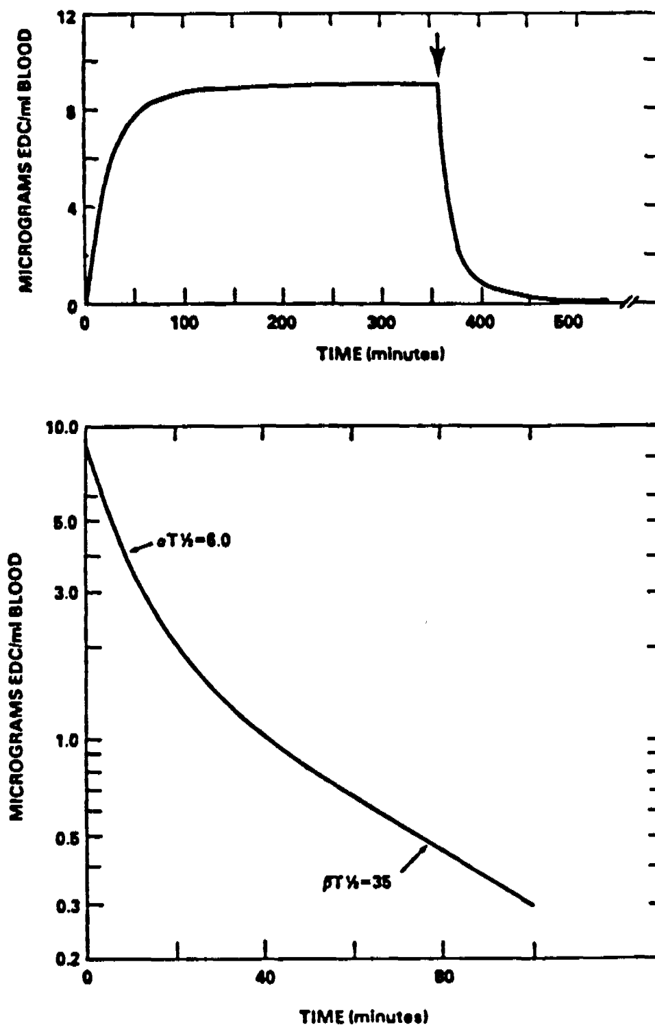
Figure 9-2. Top: Blood levels of EDC observed during and following a 6-hour inhalation exposure to 150 ppm EDC. Data from four male Osborne-Mendel rats were fitted to a two-compartment open model as described by Gehring et al. The computer plot is shown. The arrow indicates exposure termination. Bottom: Semi-logarithmic plot of EDC blood levels vs. time after exposure termination.
