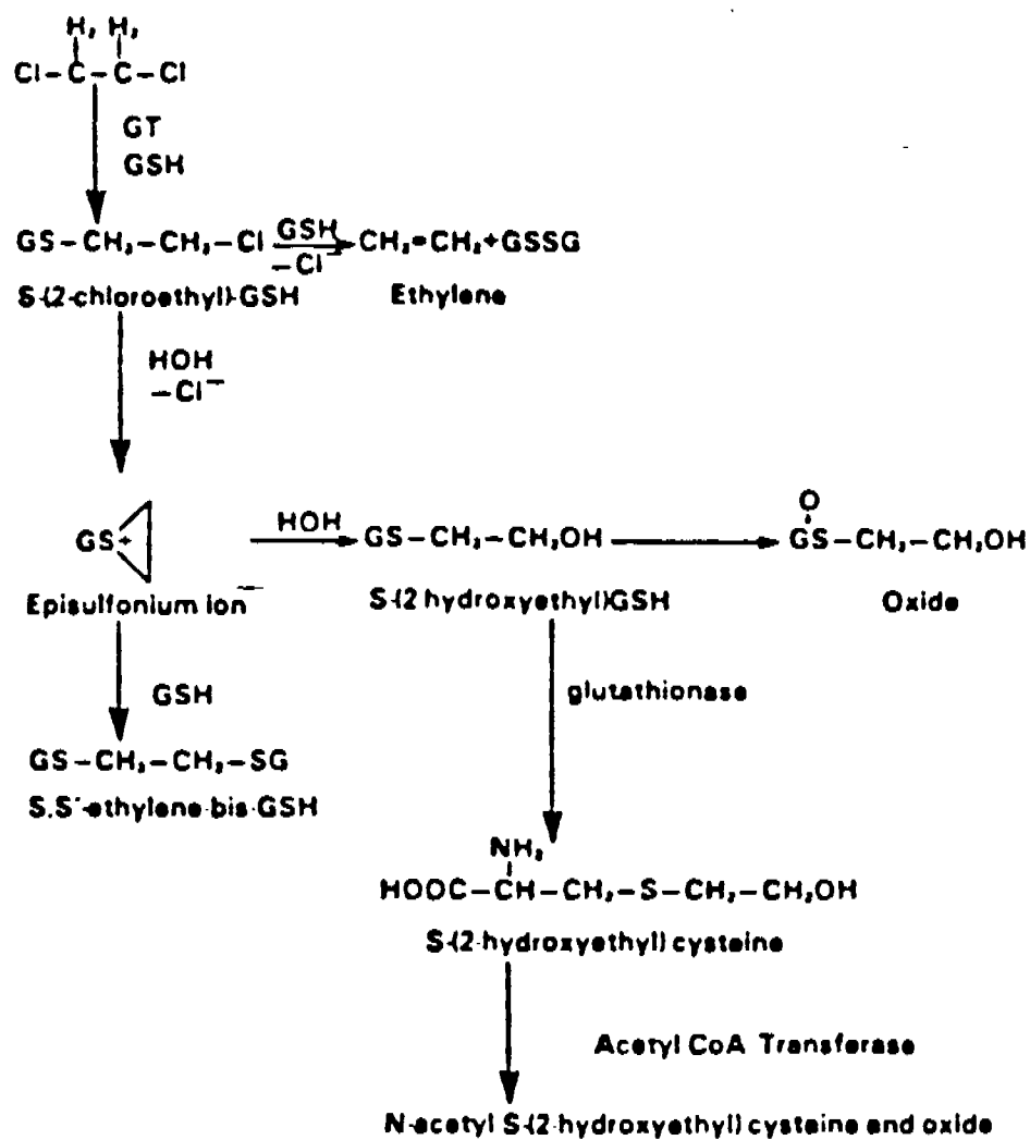
Figure 9-7. Postulated cytosolic metabolism of ethylene dichloride.
