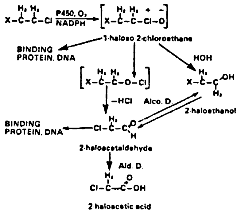
Figure 9-5 Postulated microsomal oxidative metabolism of 1,2-dihaloethanes.
