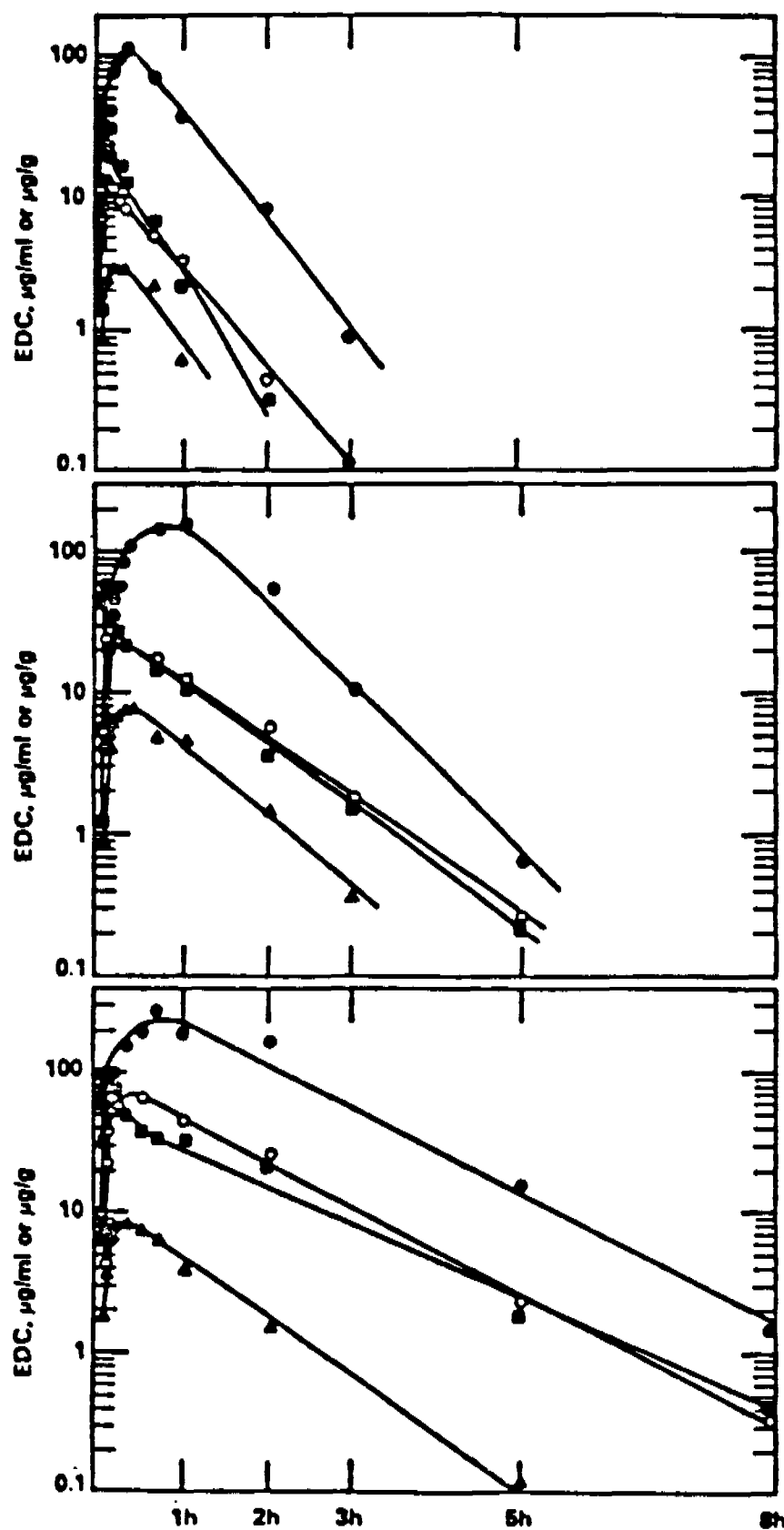
Figure 9-1. EDC levels after single oral administration in rats: Top panel, 25 mg/ kg; middle, 50 mg/kg; bottom, 150 mg/kg dose. Adipose tissue ( \circ ), blood ( \square ), liver ( \blacksquare ), lung ( \blacktriangle ).
