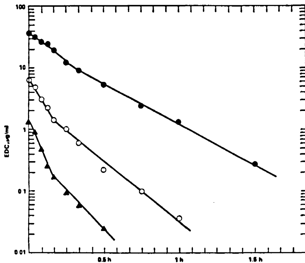
Figure 9-3. Blood levels of EDC in rats after i.v. administration. (●) 25 mg/kg i.v.; (○) 5mg/kg i.v.; (▲) 1 mg/kg i.v.
