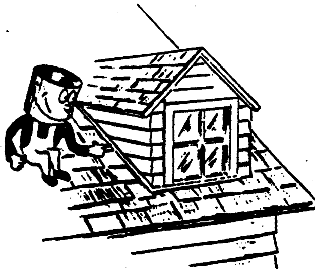
Figure 4.—Method of fitting dormer siding to roof to protect siding ends from water. Metal flashing extends back of siding and under shingles.
