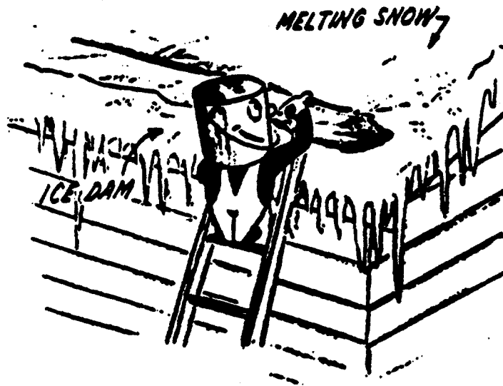
Figure 7.—How ice dams form. Snow water from upper roof freezes on cold overhang or in snow-clogged gutters, builds up dam.
