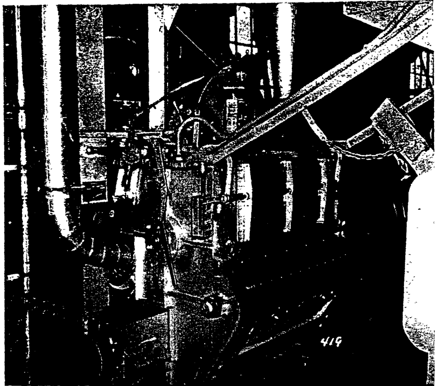
Figure 6. A tumbling barrel used for finishing small castings. The barrel is in operation, but note the absence of dust due to a good exhaust system.
