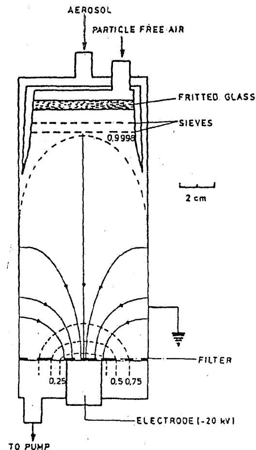
Fig. 3. System of Zebel and Hochrainer (63) for separating fibres and isometric particles. The electric field ( -20 \text{ kV} ) lines of force are marked with arrows. They cross the air flow lines which are vertically downwards and draw the charged particles from the periphery to the centre of the filter. Fibres carry greater charges than compact particles and are found closer to the centre.
