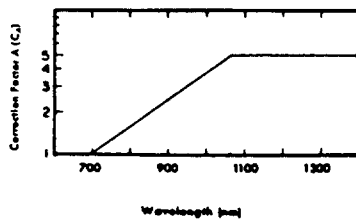
Figure 2 — TLV correction factor for \lambda = 700 - 1400 \text{ nm}
