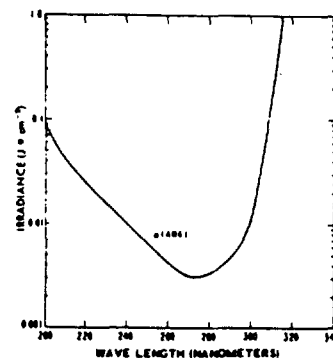
Figure 8 — Threshold Limit Values for Ultraviolet Radiation
