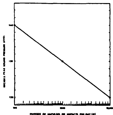
Figure 7 — Threshold Limit Values for Impulse/Impact Noise.
