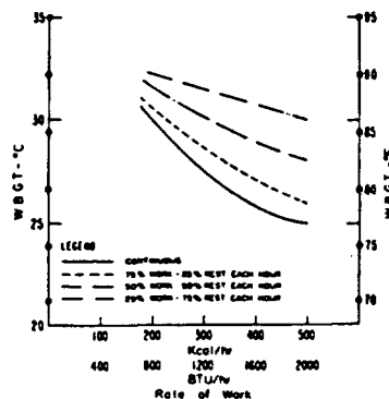
Figure 1 — Permissible Heat Exposure Threshold Limit Value
