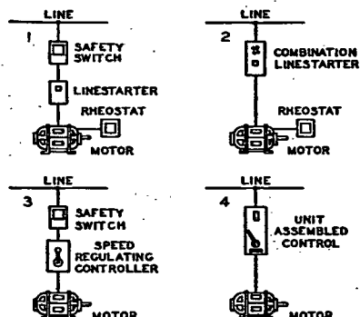
FIG. 5. RECOMMENDED CONTROLS FOR WOUND ROTOR MOTORS
