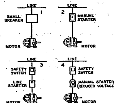
Arrangements 2, 3 and 4 are optional for motors up to 7\frac{1}{2} hp, 220 volts.
