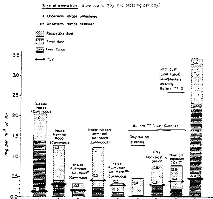
Figure 5. Comparison of mean concentration of dust in \text{mg}/\text{m}^3 of air, fraction of free-silica and TLV, in personal gravimetric samples collected at the breathing zone of sandblasters wearing various types of protective hoods.
