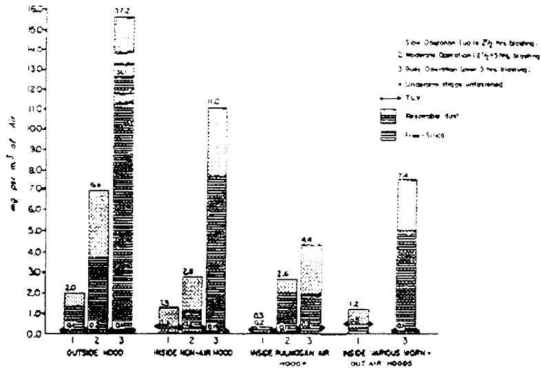
Figure 4. Comparison of mean concentration of respirable dust in \text{mg}/\text{m}^3 of air, fraction of free-silica and TLV in personal gravimetric samples collected outside hoods and inside various types of hoods.
