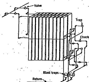
FIG. 12. SUPPLY AND RETURN CONNECTIONS FOR HEATING UNITS OF CENTRAL FAN SYSTEMS
