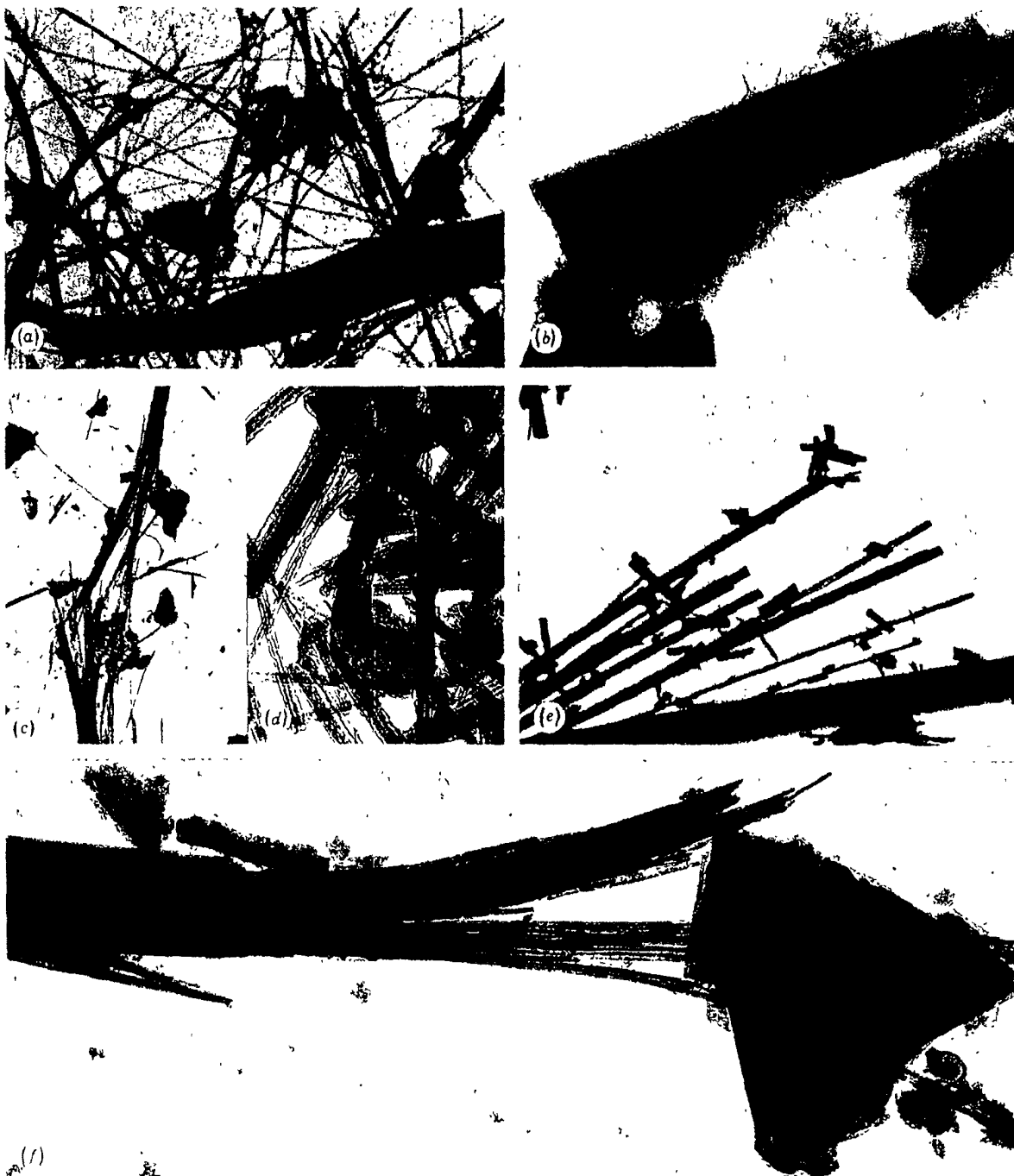
FIGURE 6. Mineral particles in leisure and domestic articles. (a) Chrysotile in papier maché; magn. \times 4500 (b) Amphibole in children's modelling compound, magn \times 17000 . (c, d) Chrysotile in plaster patching compounds, magn \times 10000 , \times 100000 . (e) Tremolite fibres in vermiculite; magn. \times 10000 . (f) Chrysotile fibre bundles in vermiculite; magn. \times 40000 .
