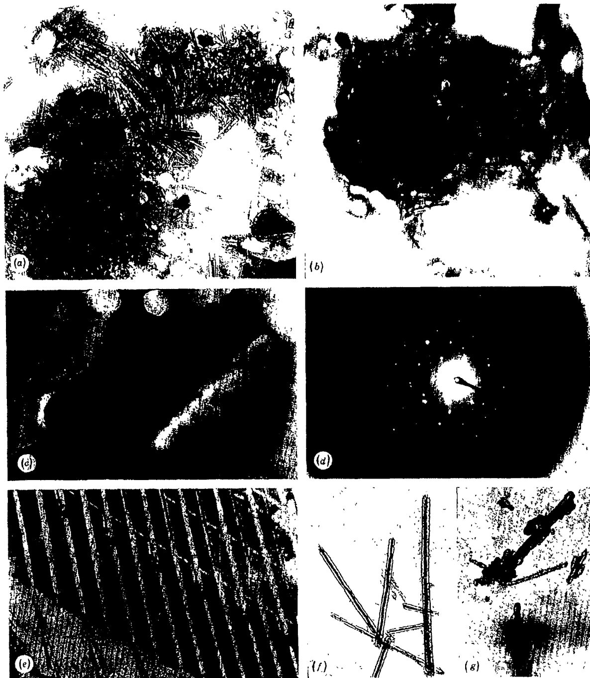
FIGURE 1 Mineral particles in the atmosphere. (a) Chrysotile in Greenland ice cap 1750, magn \times 55000 . (b) Chrysotile in Greenland ice cap 1920; magn \times 40000 . (c) Amphibole in Greenland ice cap 1920, magn. \times 20000 . (d) Selected area electron diffraction pattern of amphibole in (c). (e) Asbestos spray clouds at construction site, New York City. (f, g) Chrysotile in indoor air samples, New York City; magn \times 19000 , \times 15000 .
