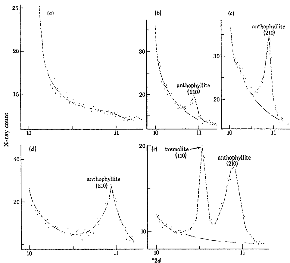
FIGURE 8. X-ray diffraction step scans of talc samples. ( a, b, c ) Representative dilution standards containing 1 %, 5 % and 10 % anthophyllite in talc. ( d, e ) Consumer talcum powders purchased in New York City.
