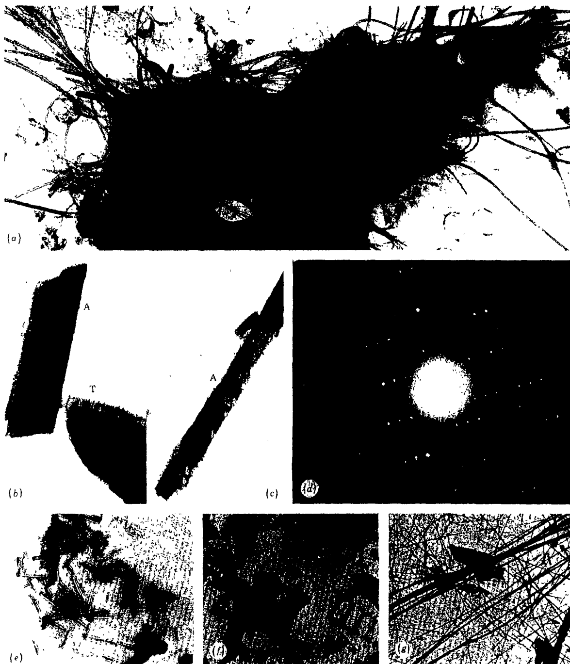
FIGURE 4. Mineral particles in water, food, drugs, tobacco sheet and clothing. (a) Chrysotile in water, Thetford, Canada; magn. \times 40\,000 (b, c) Amphibole (A) and talc (T) on rice; magn \times 20\,000 , \times 15\,000 . (d) Selected area electron diffraction pattern of amphibole in (c). (e) Asbestos in parenteral drug; magn. \times 30\,000 . (f) Diatom fragments and short fibres (arrowed) in low temperature ashed reconstituted tobacco sheet; magn. \times 3000 (g) Chrysotile present (8%) in a woman's coat; magn. \times 2250 .
