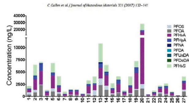
Fig. 1. Mean concentrations (ng/L) of investigated nine PFASs in 27 landfills across Australia.
