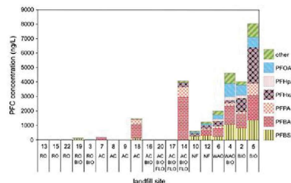
Fig. 1. PFC concentrations in treated leachate of 19 landfill sites. Shown are the six most abundant compounds in ng/L. Note: Other PFCs are aggregated as 'other'. The abbreviations correspond to the treatment system of the landfill site: AC = activated carbon, BIO = biological treatment, FLO = flotation, NF = nanofiltration, RO = reverse osmosis, WAO = wet air oxidation.
