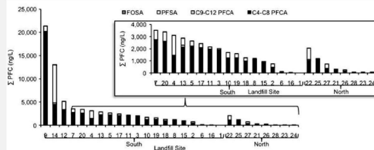
Fig. 2 Total PFC concentrations in landfill leachate across Canada. The bars represent the sum of the four sub-groups of PFCs
