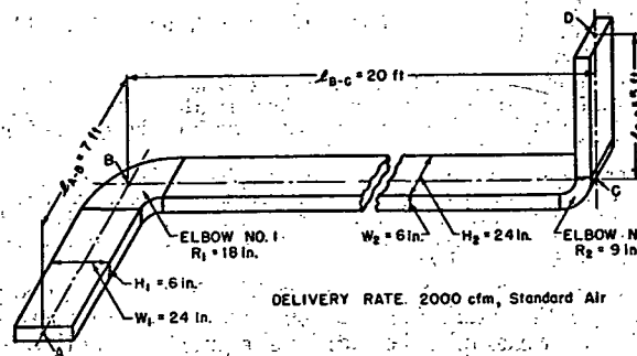
FIG. 7. PORTION OF DUCT SYSTEM FOR EXAMPLE 3
