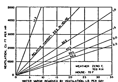
Fig. 7 .... Water Vapor Balance in a Dwelling
