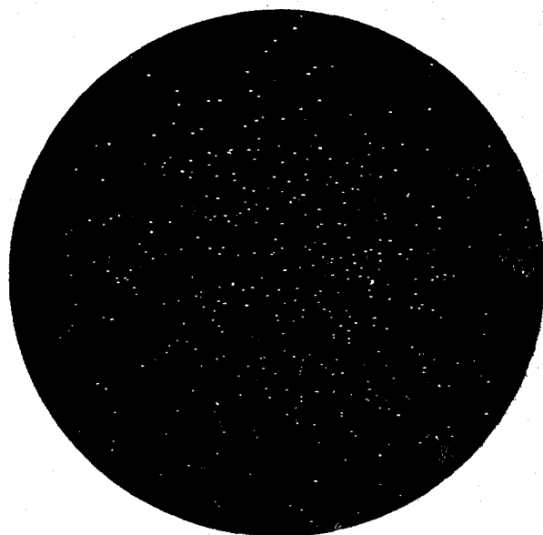
Photo of test sheet showing pattern made by Lawrence Brand No. 7½ Chilled Shot at a distance of 40 feet. (Actual diameter of test sheet: 24".)
