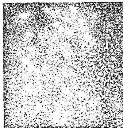
Fig. 1. Holes in a cellulose nitrate film produced by bombardment with 3 Mev \alpha -particles followed by a 3-minute etch in 6N NaOH aqueous solution at 75°C.
