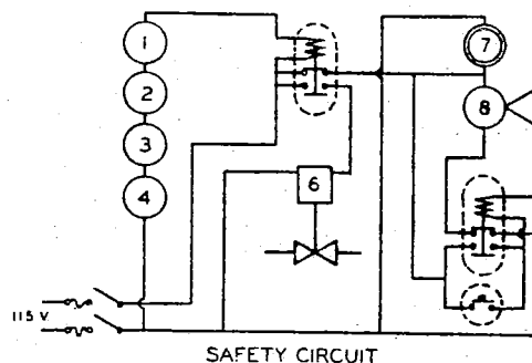
Figure 3. Control and Safety Circuit
