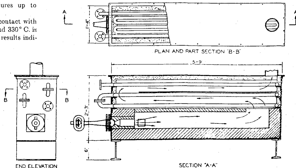
Figure 1. Heater
