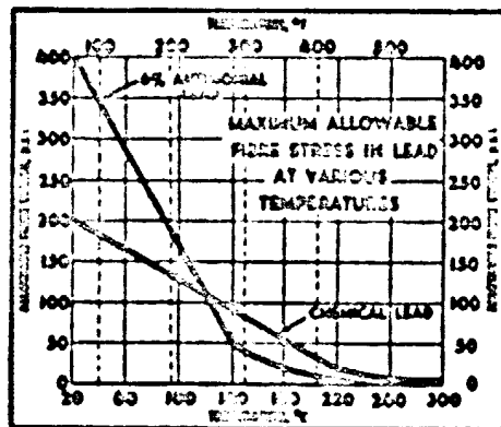
Figure 7. Maximum allowable fibre stress in chemical and 6 percent antimonial lead at various temperatures. Fifty pound saturated steam lines on at 140° C (284° F).
