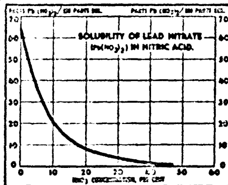
Figure 2 Solubility of lead nitrate (Pb(NO 3 ) 2 ) in nitric acid. Parts of lead nitrate per 100 parts of solution are plotted against nitric acid concentration in percent.
