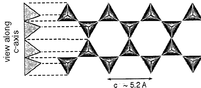
Figure 1: Amphiboles consist of double chains of silicate tetrahedra aligned along the c-axis of the unit cell.
