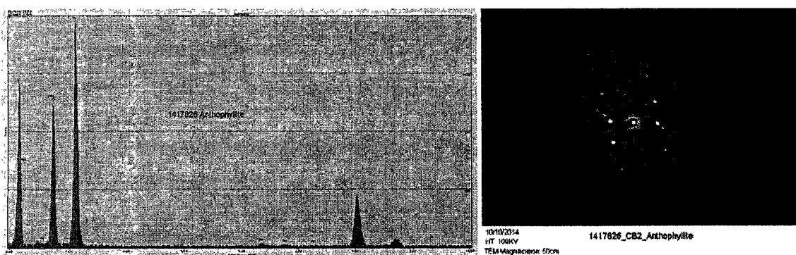
Figure 19: TEM EDS showing consistent chemistry with anthophyllite and SAED confirming crystalline structure of anthophyllite asbestos in Cashmere Bouquet talcum powder product received from Simon Greenstone Panatier Bartlett September 12, 2014.
