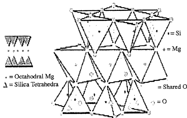
Figure 2: Talc consists of silica tetrahedra in a sheet, with magnesium sandwiched in a molecular arrangement called "octahedral coordination" by dint of the sharing of oxygens in 6 corners. Notice the hexagonal ring formed by the silica tetrahedra (as viewed from above).
