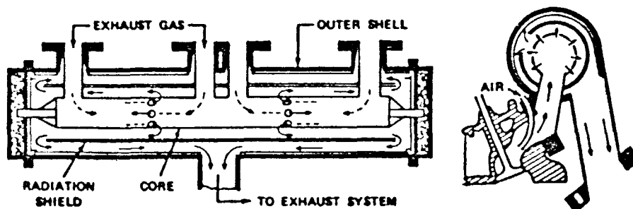
Type V Shielded Exhaust Manifold Reactor.
