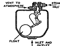
FIG. 35. BOILER RETURN TRAP OR ALTERNATING RECEIVER
