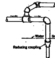
FIG. 36. DRIFTING MAIN WHERE IT RISES TO HIGHER LEVEL
