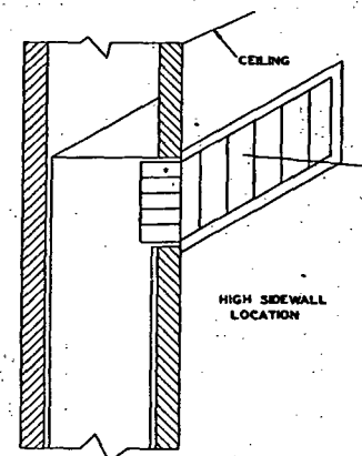
FIG. 2. RECOMMENDED TYPE OF HIGH SIDEWALL INSTALLATION ON WARM WALL a
