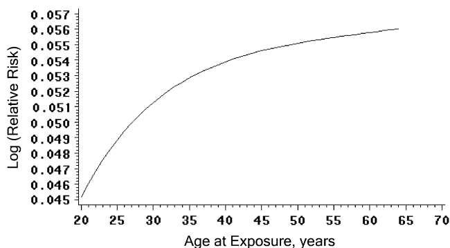
Figure 3. Relative risk of leukemia by age at exposure to benzene. Impact of a single year of exposure at 10 parts per million for a rubber hydrochloride worker aged 65 years, Ohio, 1940–1996.
