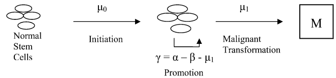
Figure 1. Pictorial depiction of the 2-stage clonal expansion model. Refer to the Materials and Methods section of the text for an explanation of the parameters.
