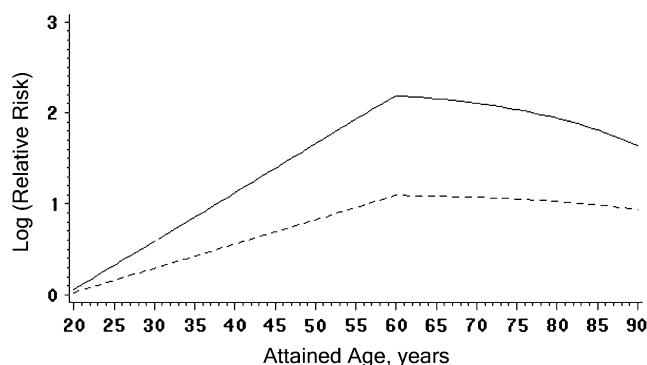
Figure 2. Relative risk of leukemia by attained age. Predicted impact of benzene exposure for rubber hydrochloride workers in Ohio (1940–1996) at intensities of 5 parts per million (dashed line) and 10 parts per million (solid line) based upon fitting of the 2-stage clonal expansion model. Benzene exposure commences at age 20 years and terminates at age 60 years.
