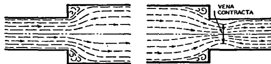
FIG. 8. AIR FLOW AT ABRUPT ENLARGEMENT OR CONTRACTION OF AIR STREAM
