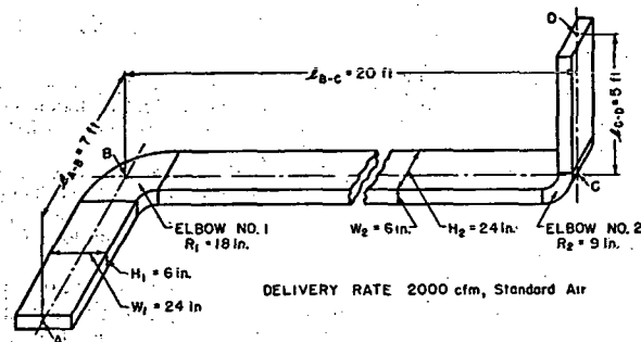
FIG. 7. PORTION OF DUCT SYSTEM FOR EXAMPLE 3
