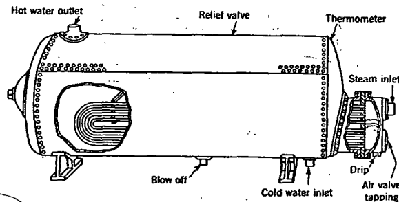
FIG. 8. INDIRECT WATER HEATER
