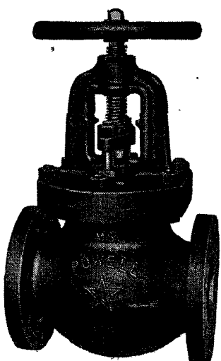
Fig. 1793—125-pound Iron Body Bronze Mounted Gate Valve for 125 pounds W. in sizes 2" to 30", incl. Has flanged end, bolted flanged yoke, outside screw rising stem and taper wedge solid disc. Taper wedge double discs can be provided in sizes 2" to 12", incl. Seat rings and stem are in bronze. Disc is bronze in 1 1/4" and smaller size valves; bronze in the larger sizes. Also available in All Iron.
