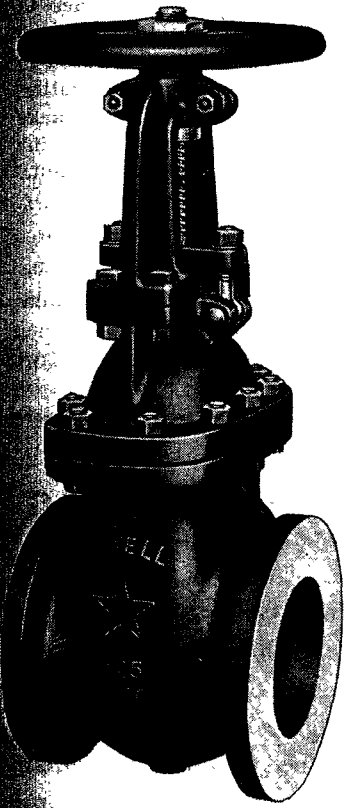
Fig. 1793—125-pound Iron Body Bronze Mounted Gate Valve for 125 pounds W. in sizes 2" to 30", incl. Has flanged end, bolted flanged yoke, outside screw rising stem and taper wedge solid disc. Taper wedge double discs can be provided in sizes 2" to 12", incl. Seat rings and stem are in bronze. Disc is bronze in 1 1/4" and smaller size valves; bronze in the larger sizes. Also available in All Iron.
