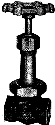
Fig. 375—200-pound Bronze Gate Valve with screwed ends, inside screw rising stem, union bonnet and renewable, wear-resisting "Powellium" nickel-bronze taper wedge solid disc in sizes 1/4" to 3/4", inclusive; taper wedge double disc in sizes 1" to 3", inclusive.
