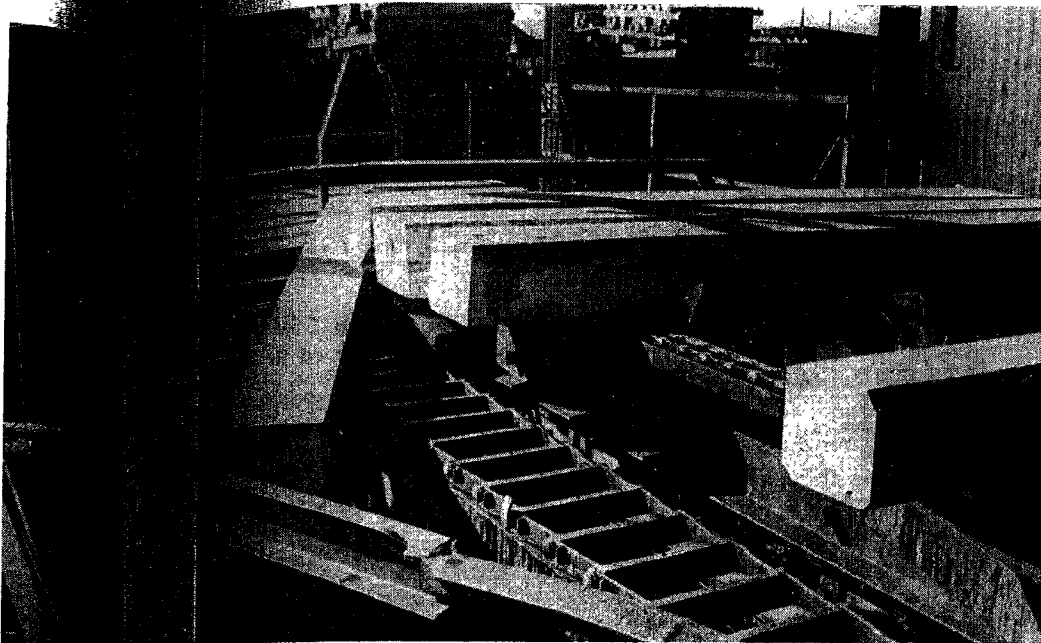
FIG. 5. ABOVE, THE SPACING TABLE. NOTE THE STRINGER TIE FINDING ITS WAY ALONG THE GUIDE BEING PROPELLED BY THE CHAIN SHOWN IN THE FOREGROUND. THREE TIES HAVE BEEN ASSEMBLED ON THE SPACING TABLE WITH THE SPACER IN POSITION TO RECEIVE THE FOURTH TIE.
