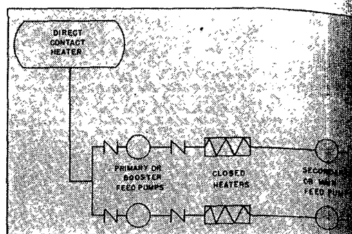
FIG. 9. WHEN BOOSTER AND MAIN FEED PUMPS ARE OPERATED AS INTEGRAL UNITS, A SINGLE BY-PASS MAY BE USED.
