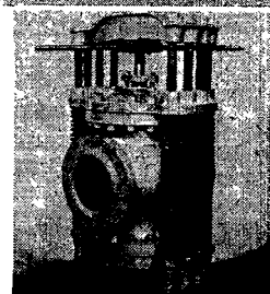
Above — No. 110 Exhaust Relief Valve for condenser protection service. Left — No. 80 "Noiseless" semi-balanced Back Pressure Valve for Exhaust lines. Right — No. 265 Turbine Bleeder and High Pressure Relief Valve.
