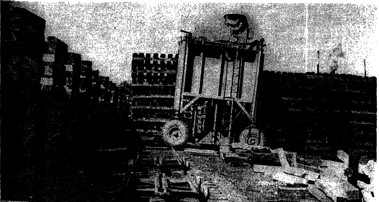
FIG. 10. THE ROSS CARRIER DESCENDS FROM THE RAILROAD TRACK AFTER PLACING A RICK OF DRY TIES (127) ON A RAILROAD TRANSFER CAR. NOTE THE MIRROR THAT IS FASTENED TO THE TOP OF THE CAR TO ASSIST THE OPERATOR.
