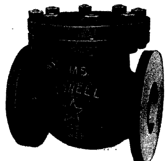
Fig. 559—125-pound Iron Body Bronze Mounted Swing Check Valve. Made in sizes 2" to 16", incl. Has flanged ends bolted flanged cap and regrindable, renewable bronze seat and disc. Disc, when wide open permits full unobstructed flow through the valve body. Also available in All Iron.
