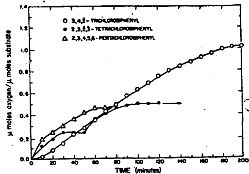
Figure 2. Oxidation of tri, tetra, and penta chlorobiphenyl.
