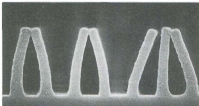
Figure 5-4 Image of line collapse that has been caused by capillary forces. 48
