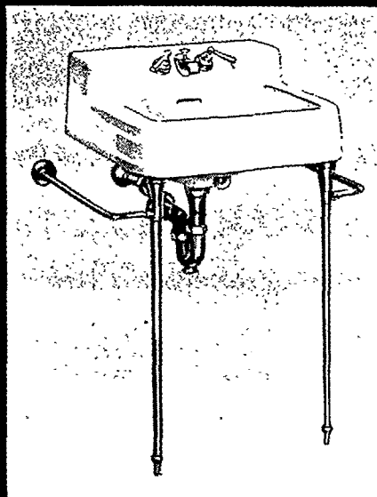
NEUDAY—C 2502 (Patented). Of porcelain enamel on cast iron and has handy shelf back. Mixing faucet gives tempered water. Sizes: 19x17 in., 24x18 in. Also made in wall hung style.
