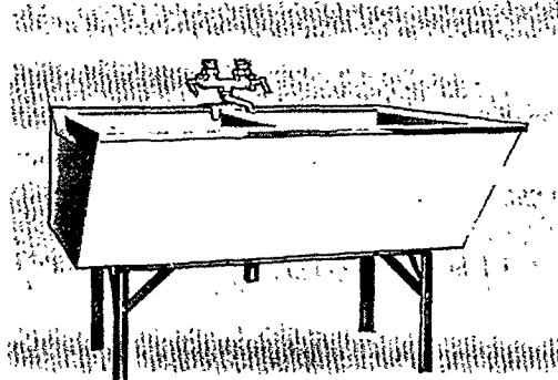
C 21294. Two-compartment cement composition laundry tub with steel supporting frame and metal rim. Sizes: 24 x 48", 54 x 24", and 60 x 24". Three-compartment style, 72 x 24".
