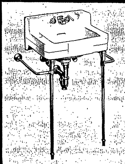
OXFORD—C 183. A compact inexpensive vitreous china lavatory. Has panel front, shelf back, mixing faucet. Comes with legs as shown, or wall hung. Size: 19x17 in.
