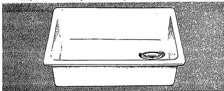
C 19350. 6" deep, flat rim sink. End outlet and Recepto waste. Sizes: 18 x 12", 20 x 14", 20 x 16", 24 x 16", 24 x 18", 30 x 18", 24 x 20", 30 x 20" and 36 x 20".
