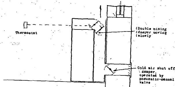
FIG. 63. DIAGRAM OF A METHOD OF CONTROL FOR A UNIT VENTILATOR
