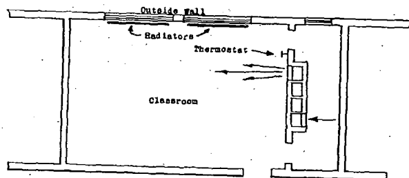
FIG. 62. PLAN OF CLASS-ROOM IN AN ELEMENTARY SCHOOL, SHOWING LOCATION OF THERMOSTAT
