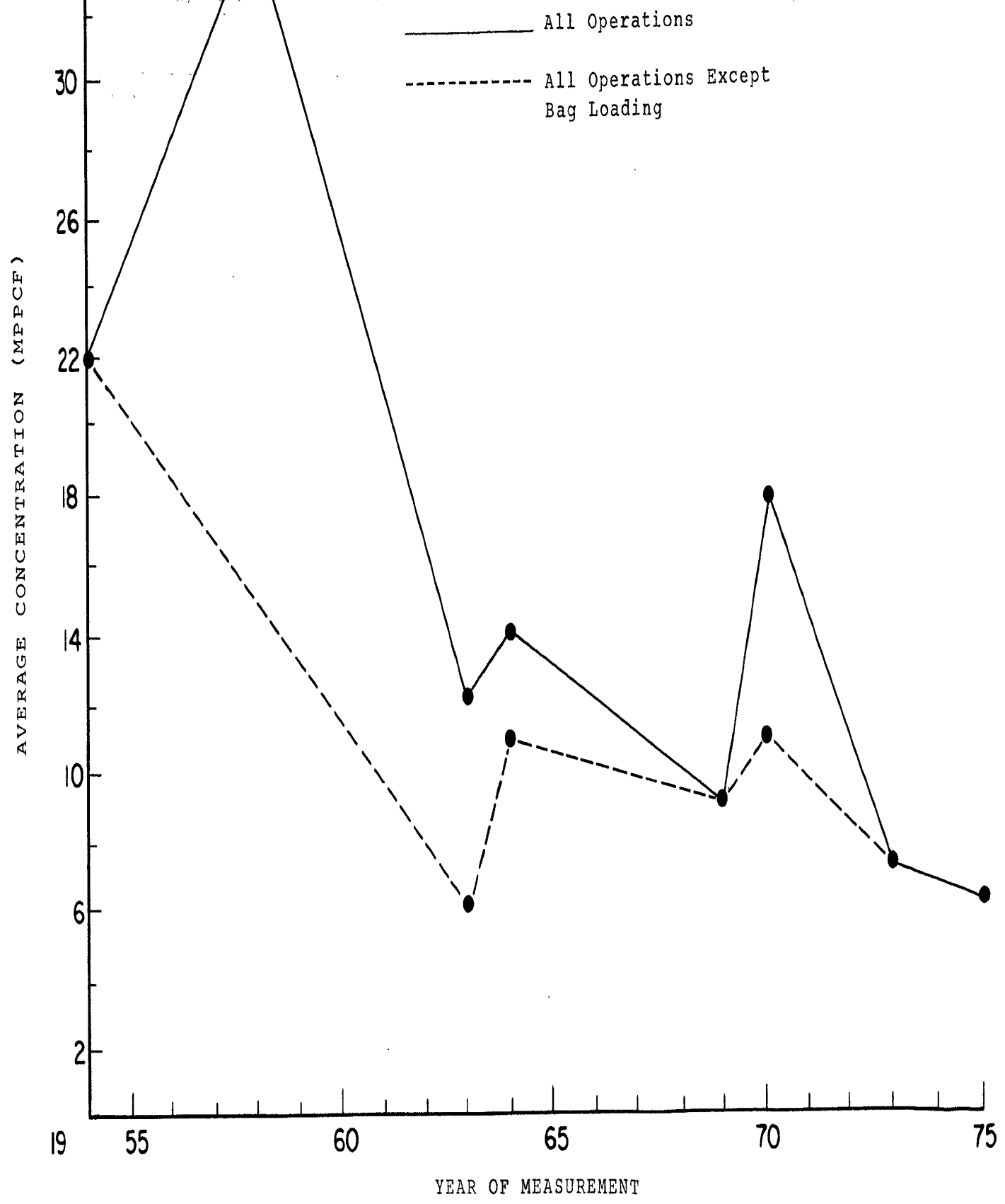
Figure 7. Mean Yearly Impinger Dust Concentrations for Mill Operations
