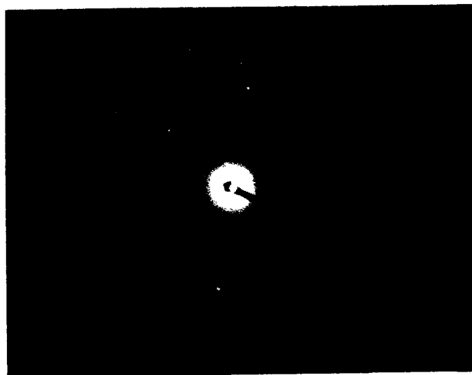
Diffraction Patterns
