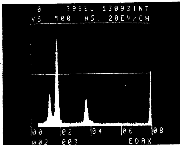
X-Ray Spectrum
