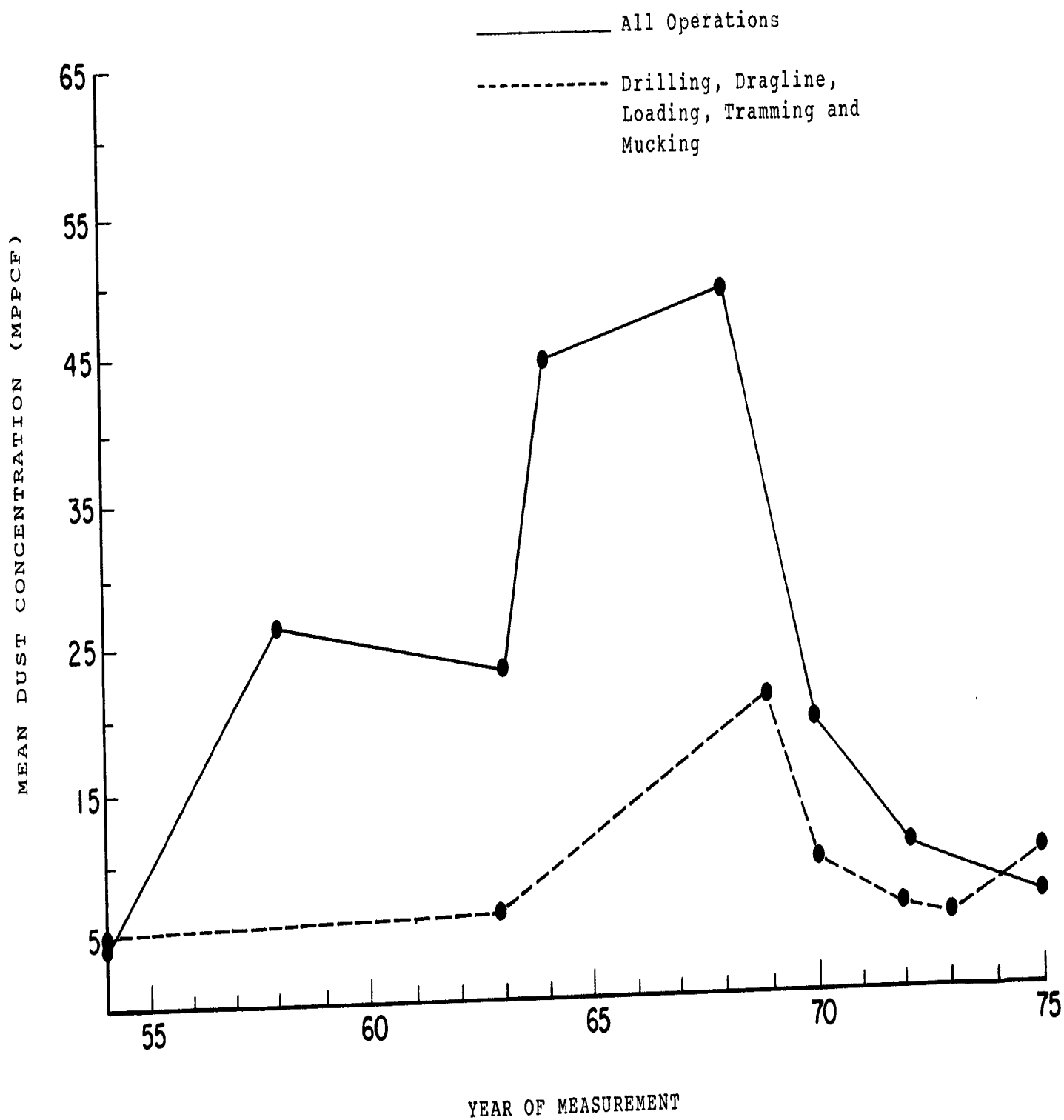
Figure 6. Mean Yearly Impinger Dust Concentrations for Mine Operations
