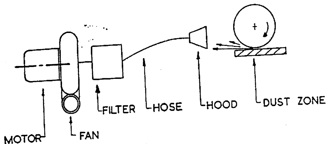
● Fig. 3—Essential components for dust extraction.
