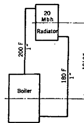
FIG. 7. GRAVITY SYSTEM
