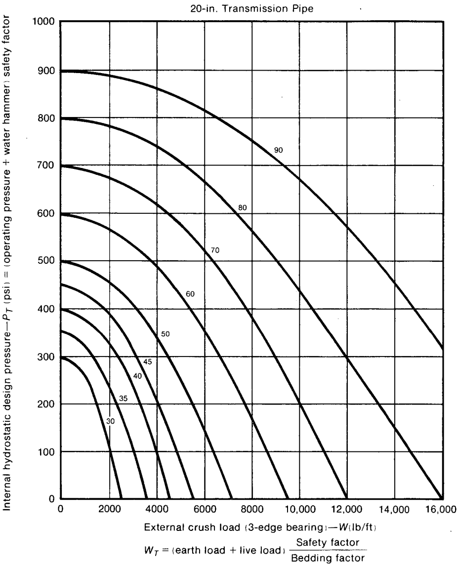
Fig. 14b. 20-in. Transmission Pipe
