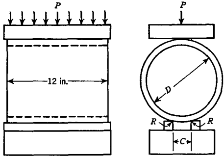
Fig. 3. Crushing Test Assembly
