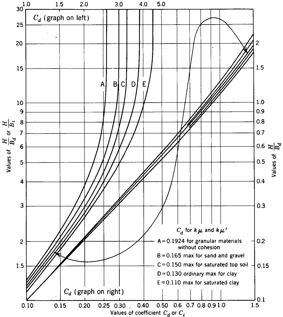
Fig. 5. Values of C_d for Trench Conditions
