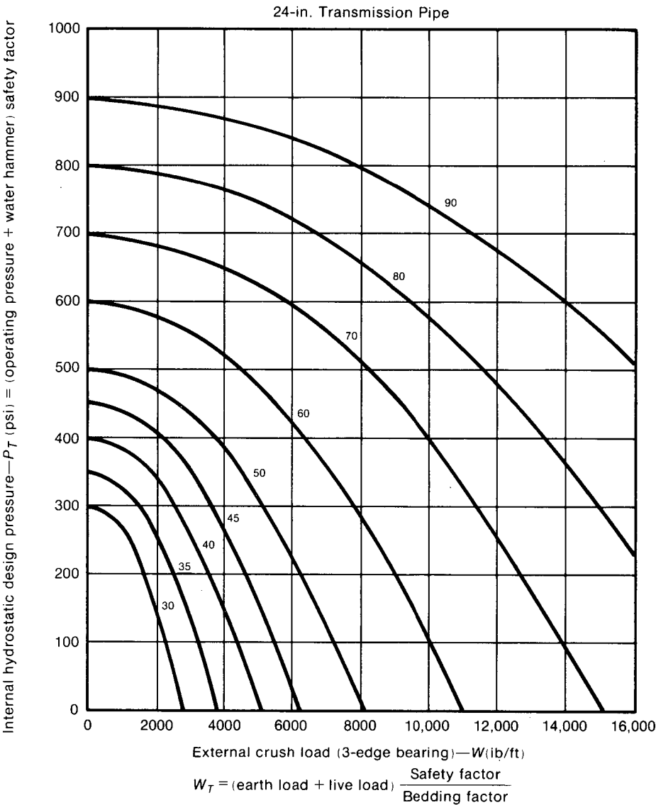
Fig. 14d. 24-in. Transmission Pipe
