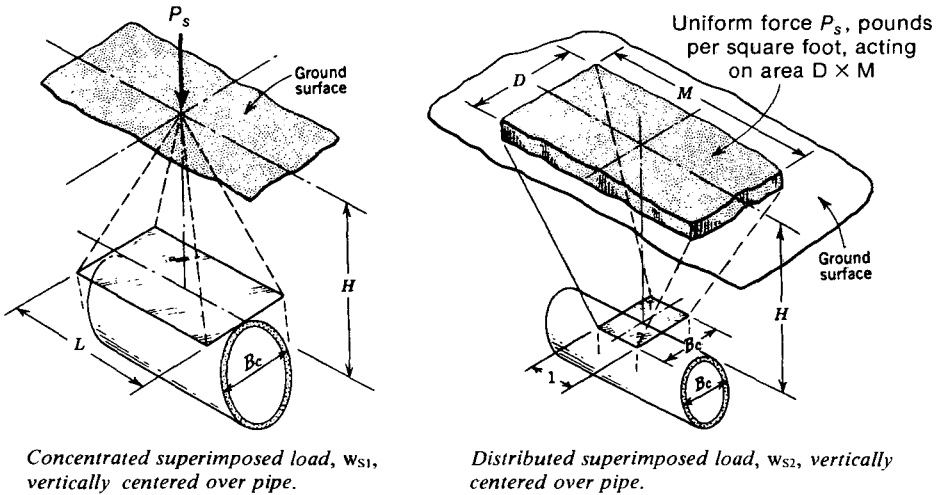
Fig. 13. Superimposed Loads
