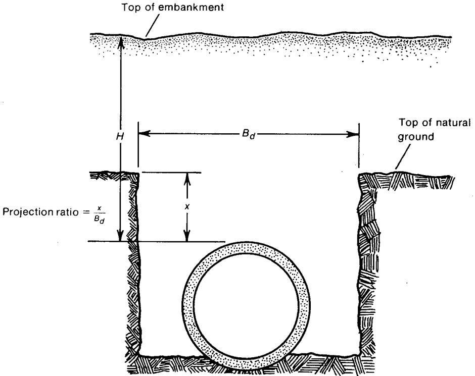
Fig. 10. Projection Ratio p for the Negative Projecting Pipe Embankment Condition
