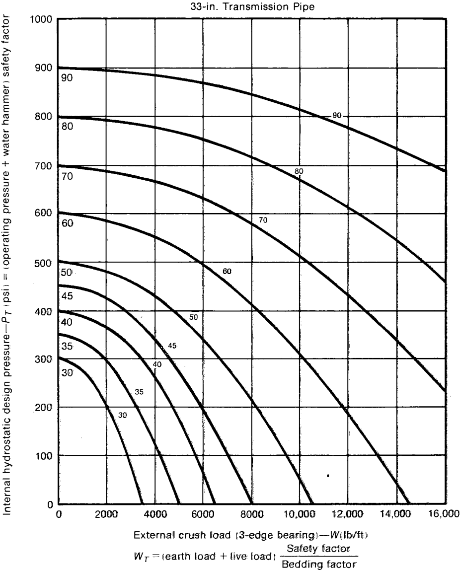
Fig. 14g. 33-in. Transmission Pipe
