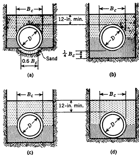
Fig. 1. Bedding Conditions
