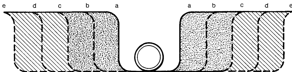
Fig. 6. Embankment Conditions
