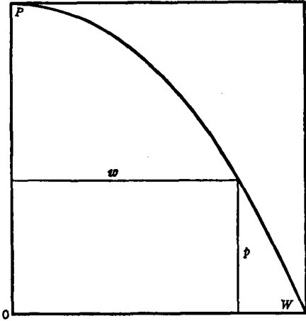
Fig. 2. Load Pressure Curve
