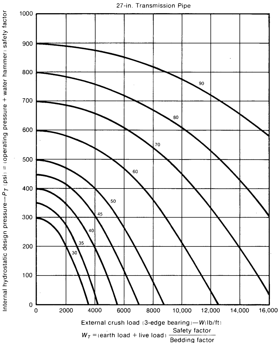
Fig. 14e. 27-in. Transmission Pipe
