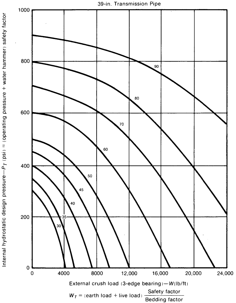
Fig. 14i. 39-in. Transmission Pipe
