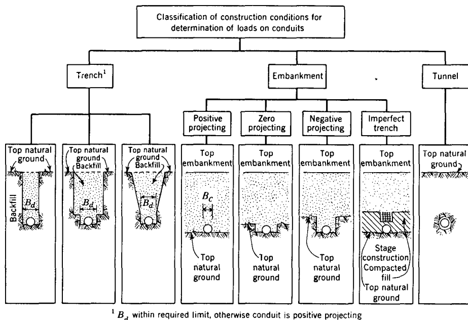
Fig. 4. Classification of Construction Techniques
