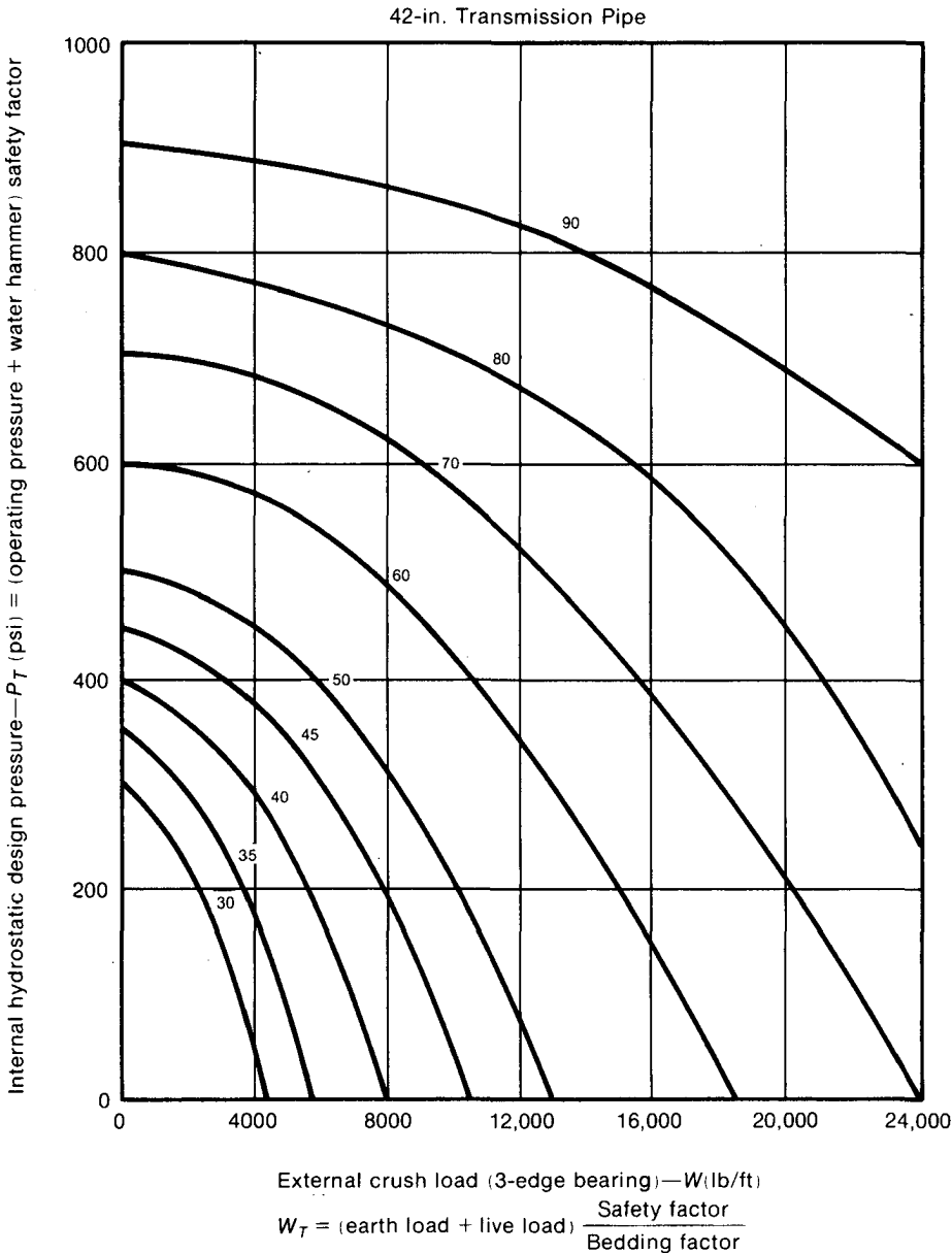
Fig. 14j—42-in. Transmission Pipe
