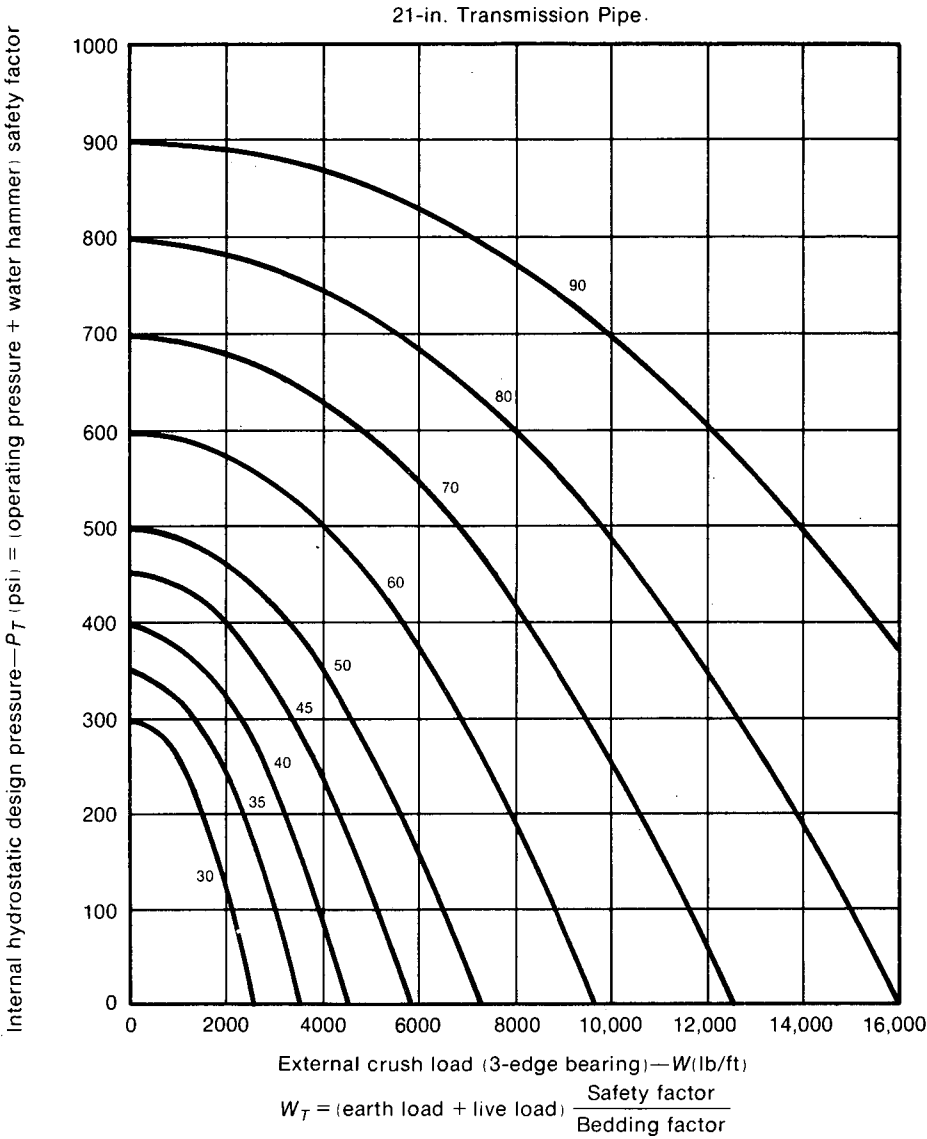
Fig. 14c. 21-in. Transmission Pipe
