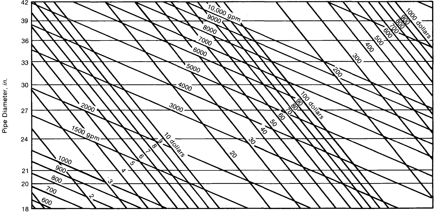
Fig. C1. Yearly Power Cost to Compensate for Friction Loss of Head * (cont. on next page)
