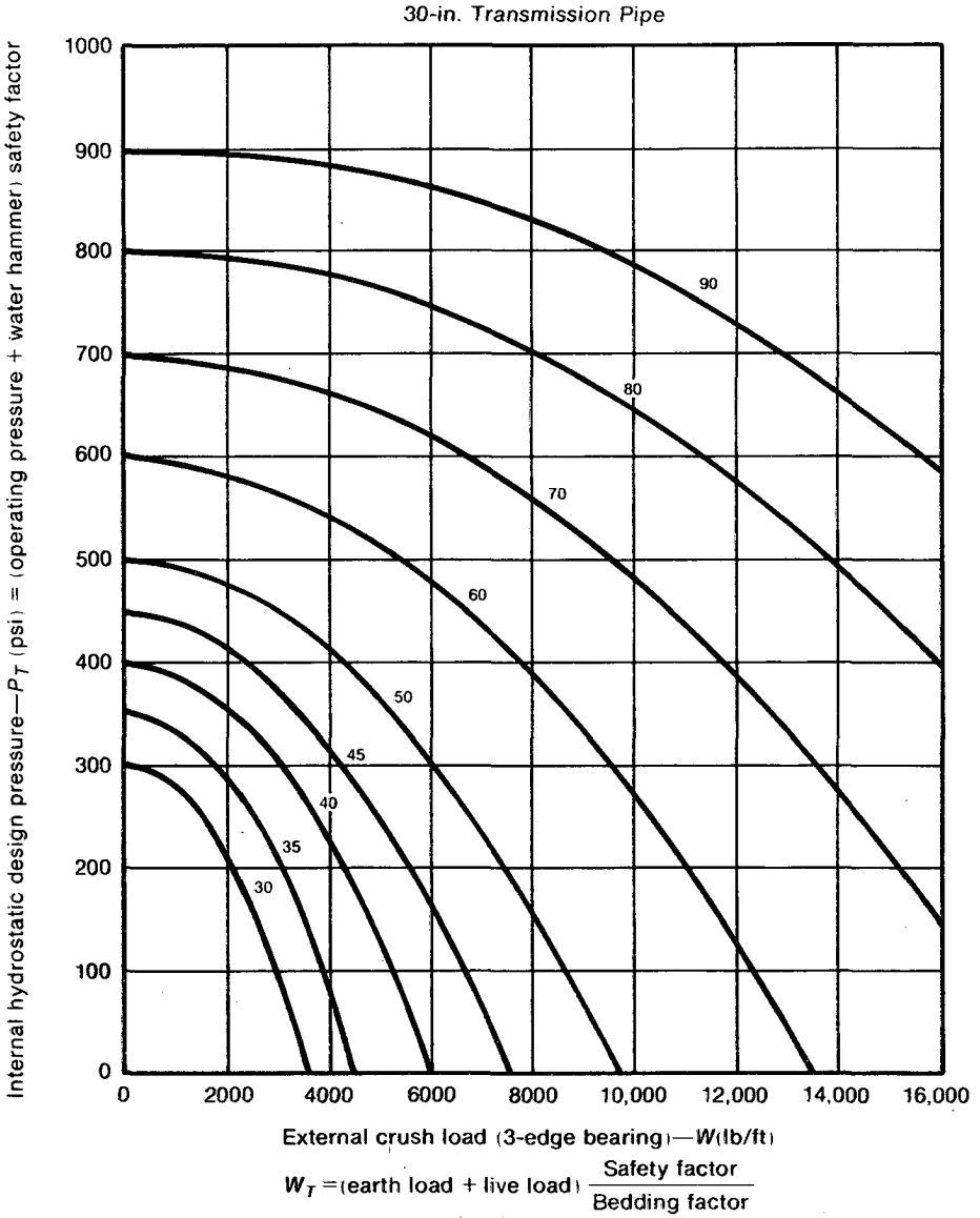
Fig. 14f. 30-in. Transmission Pipe
