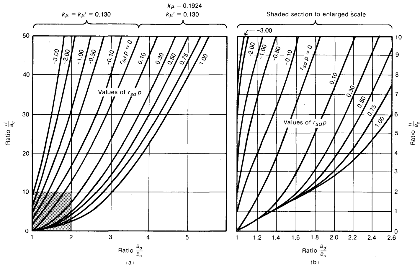
Fig. 8. Values of B_c/B_d at Which the Trench and Positive Projecting Pipe Equations Give Equal Loads
