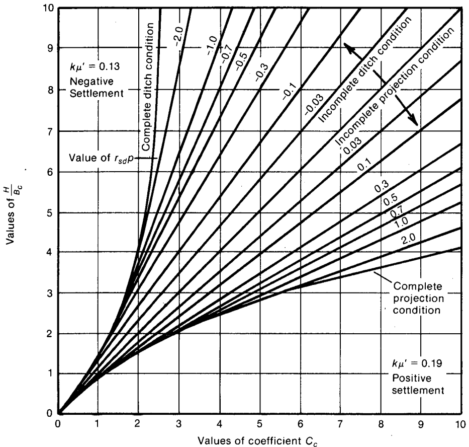
Fig. 7. Values of C_c for Positive Projecting Pipe
