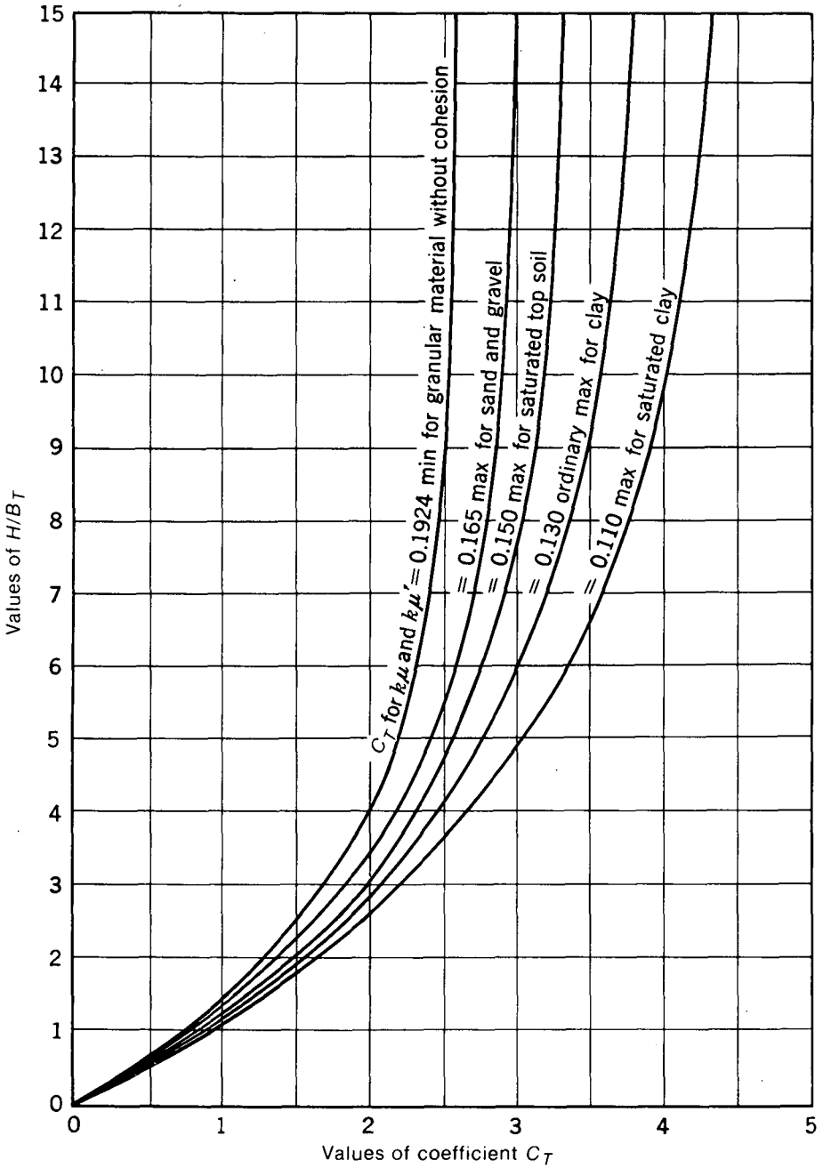
Fig. 12. Values of C_T for Tunnel Conditions
