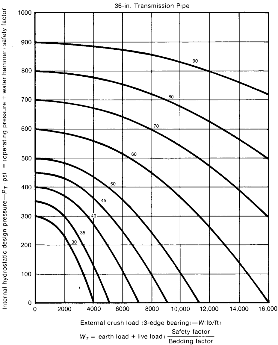
Fig. 14h. 36-in. Transmission Pipe
