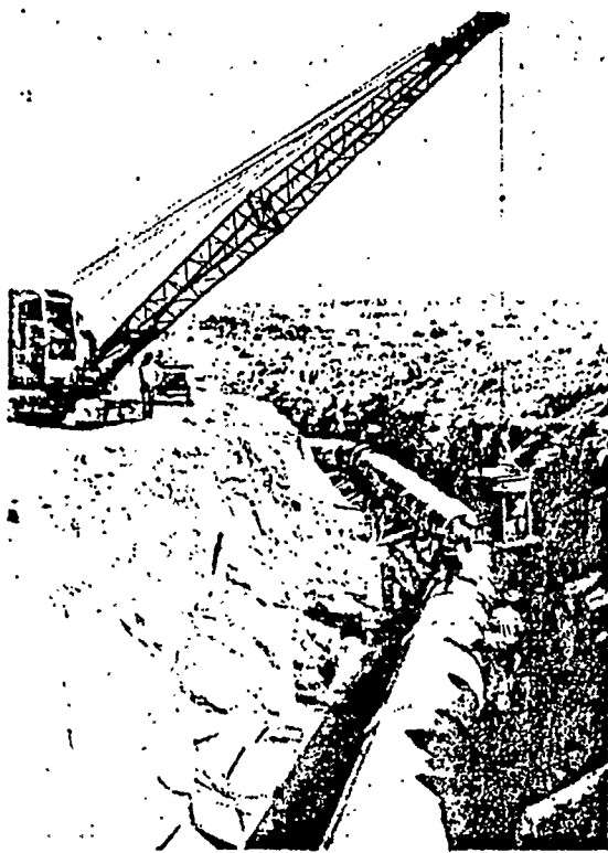
Fig. 2. A 1100-mm diameter sewer outfall in asbestos-cement is given a concrete haunching in rocky ground at Mababane in the Transvaal, South Africa.
