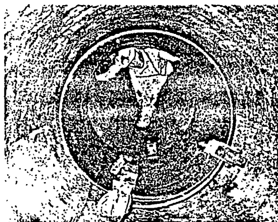
A length of RPM sewer relining prepared for grouting. The rag hanging down is a temporary plug left to allow air to escape during the grouting operation.
