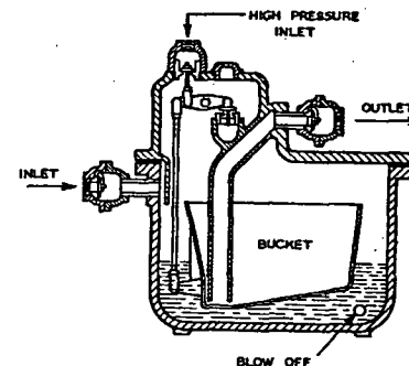
FIG. 32. LIFTING TRAP
