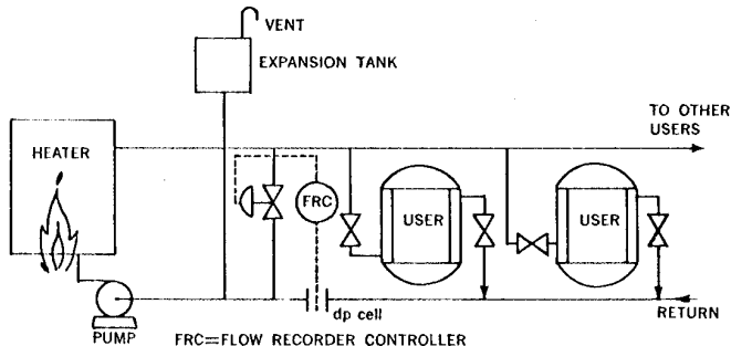
FIG. 3 FRC=FLOW RECORDER CONTROLLER WITH LOW LIMIT CUTOFF TO BURNER
