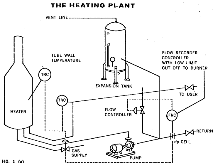
Figure 1 above illustrates a typical basic heating "plant" for a THERMINOL FR system. Note the use of instruments to control THERMINOL temperature leaving the heater and by-pass flow control to assure adequate flow through the heater regardless of "user" demands.
