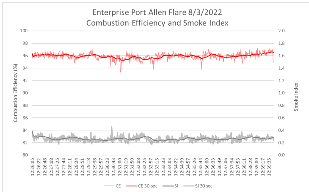
Figure 2: Combustion Efficiency and Smoke Index for the Enterprise flare on 8/3/2022.
