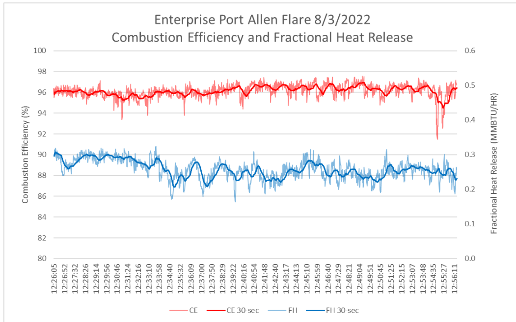
Figure 1: Combustion Efficiency and Fractional Heat Release for the Enterprise flare on 8/3/2022.
