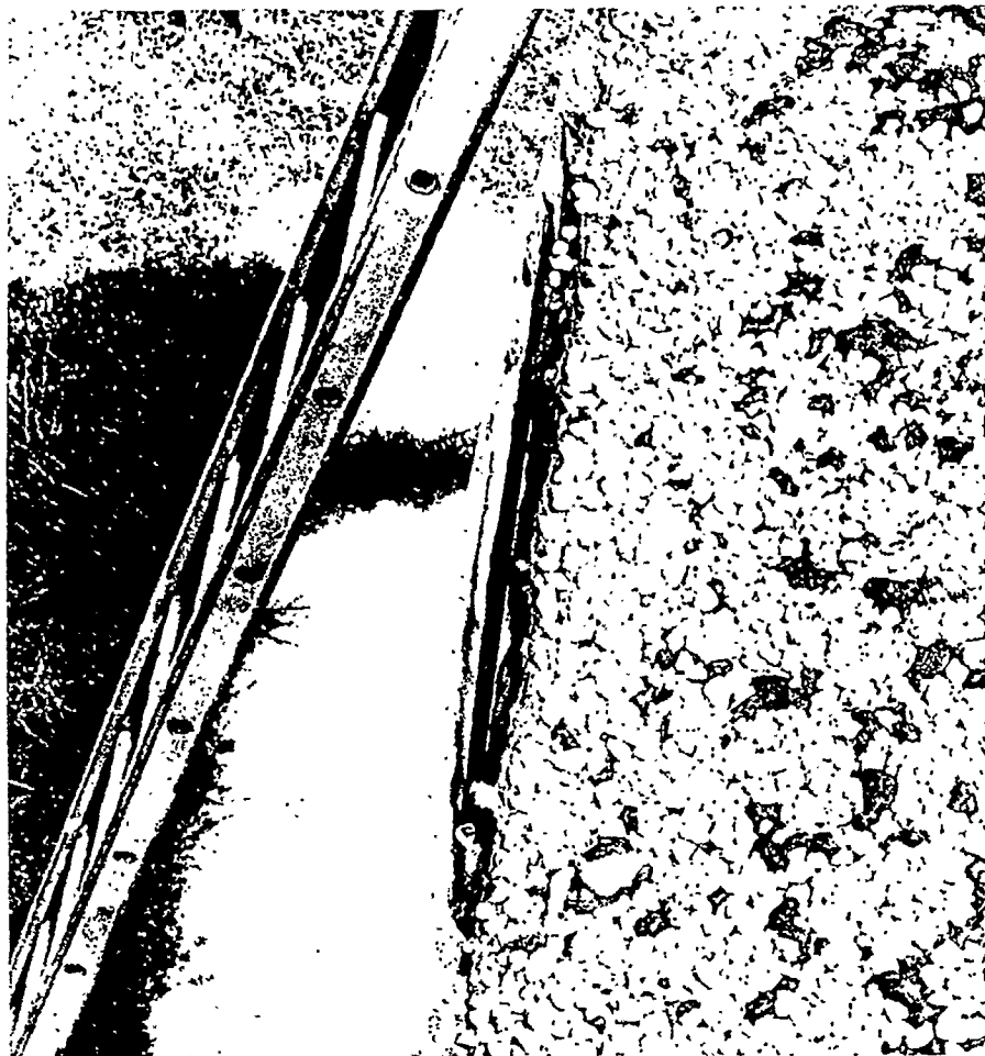
Figure 55. Deteriorated gravel stop.
