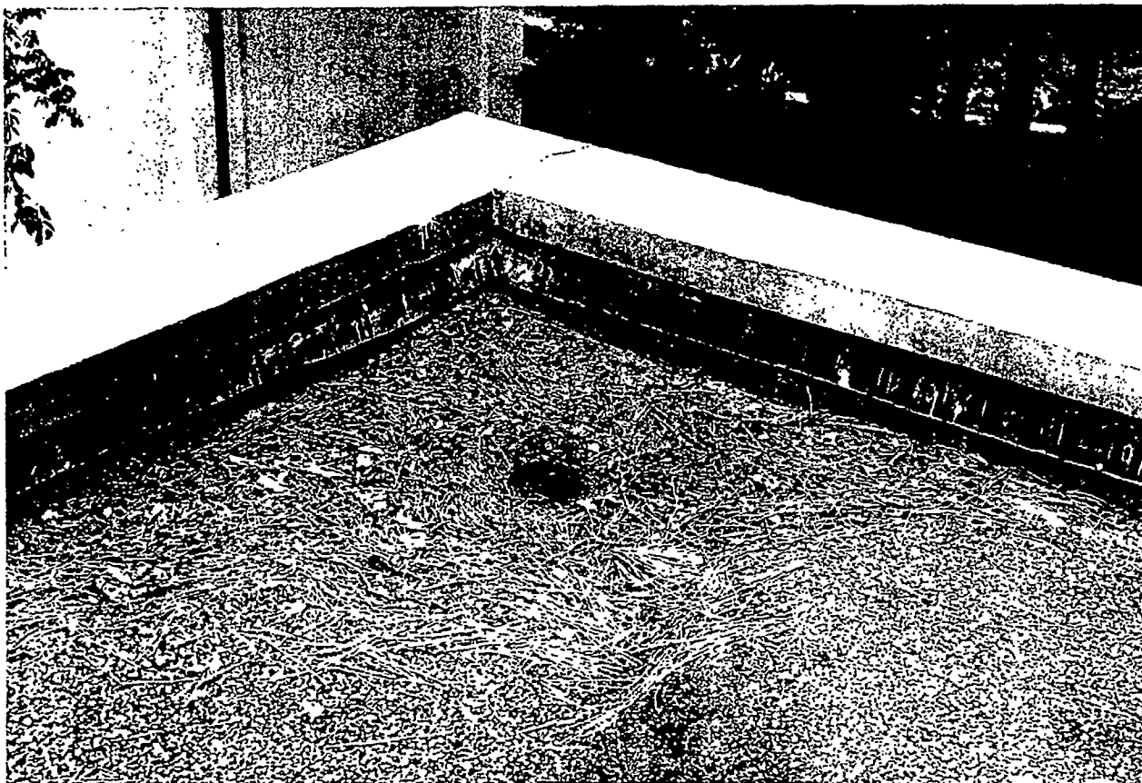
Figure 51. Debris on roof impedes drainage.
