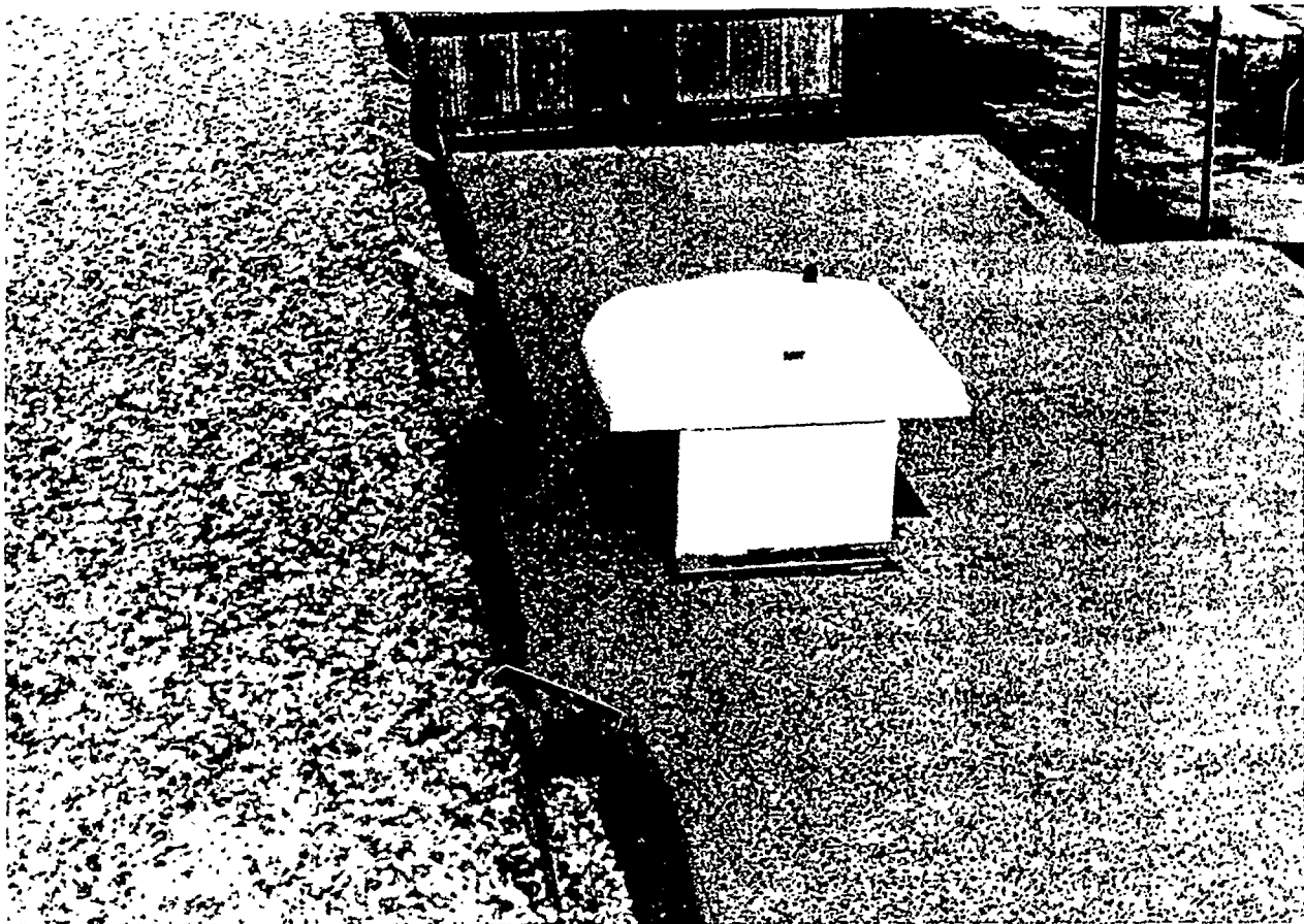
Figure 54. Accumulation of gravel causing collapse of gutter.
