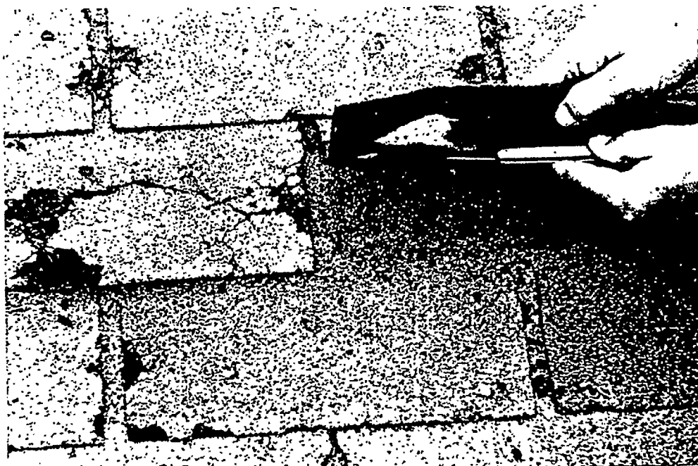
Figure 30. Hail damage showing broken shingles—reroofing mandatory.
