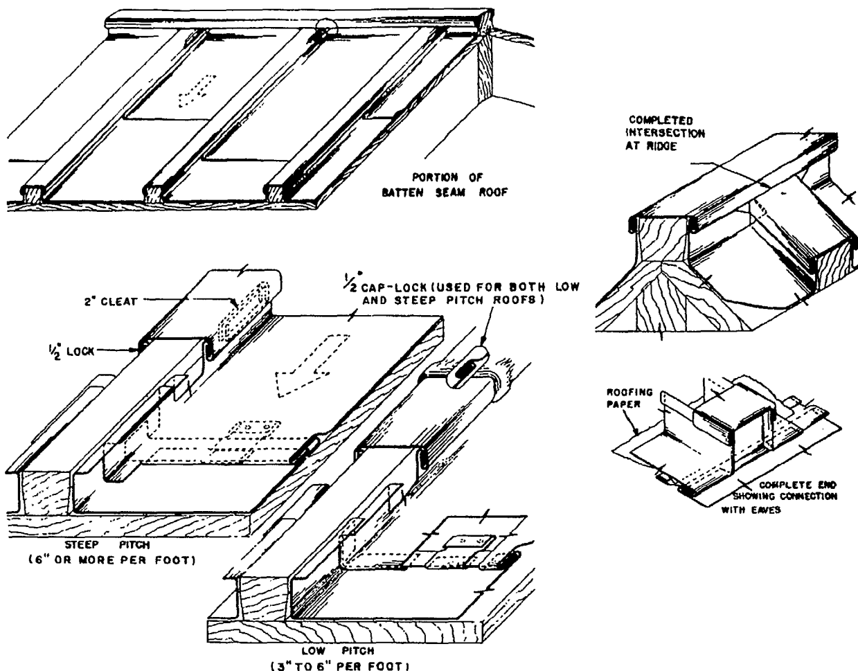
Figure 41. Batten seam roofing.
