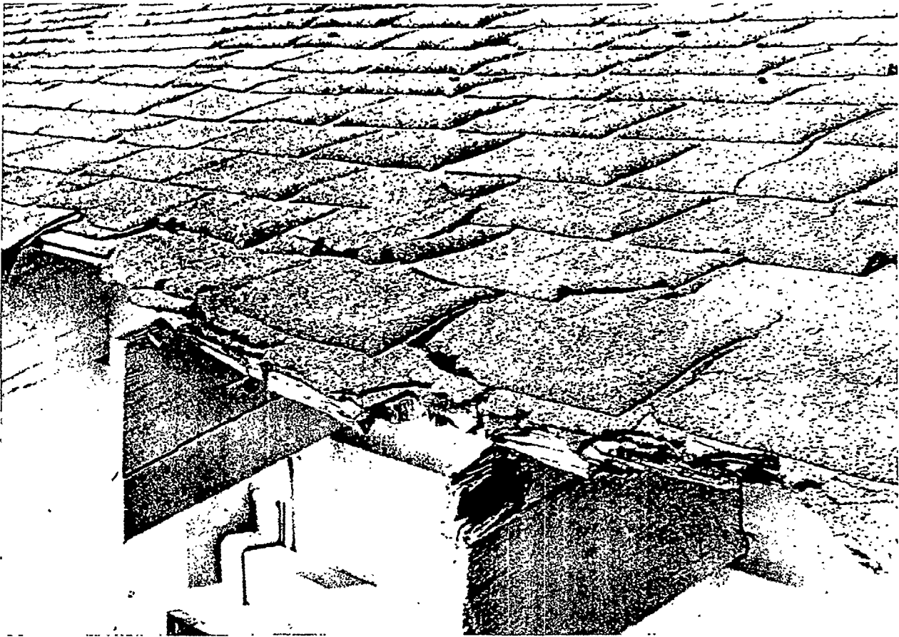
Figure 5. Inadequate provision for drip at eave—note damage to roof deck.
