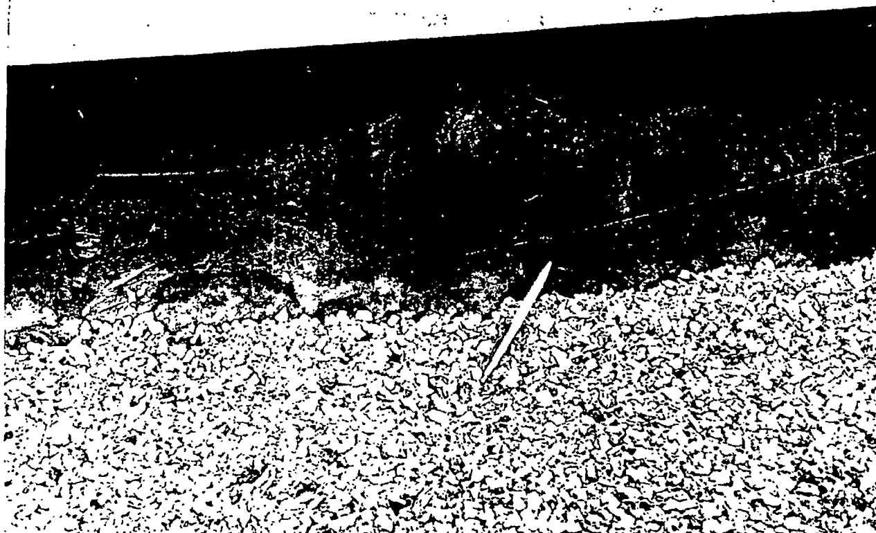
Figure 48. Puncture resulting from lack of cant strip.
