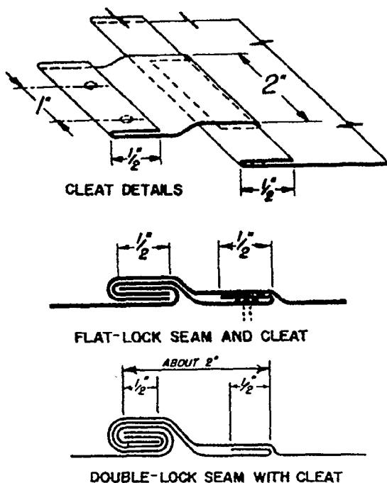
Figure 44. Typical details of cleats.
