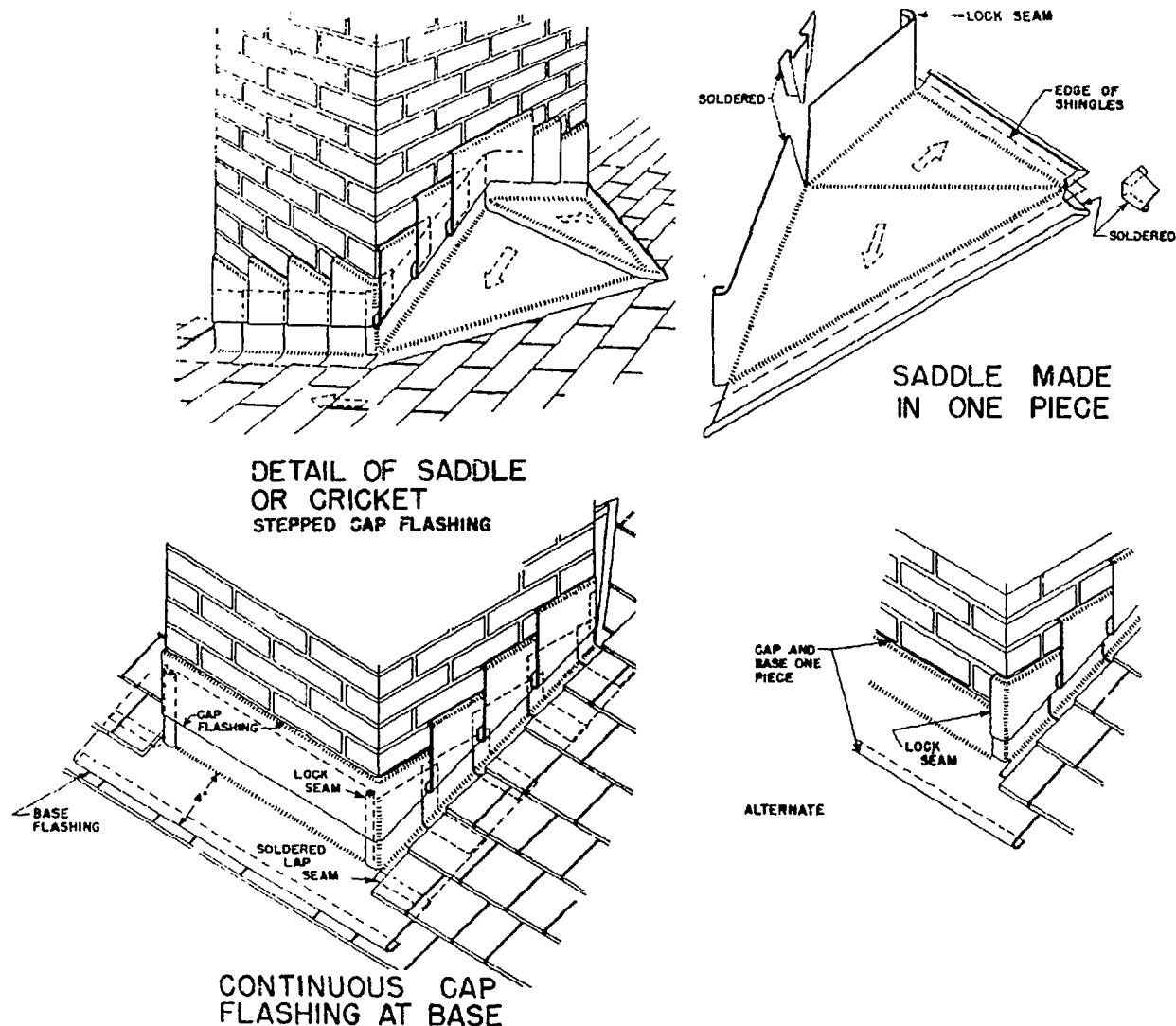
Figure 47. Typical details of chimney flashings.
