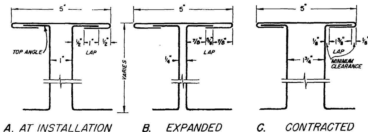
Figure 39. Movement of expansion joints.
