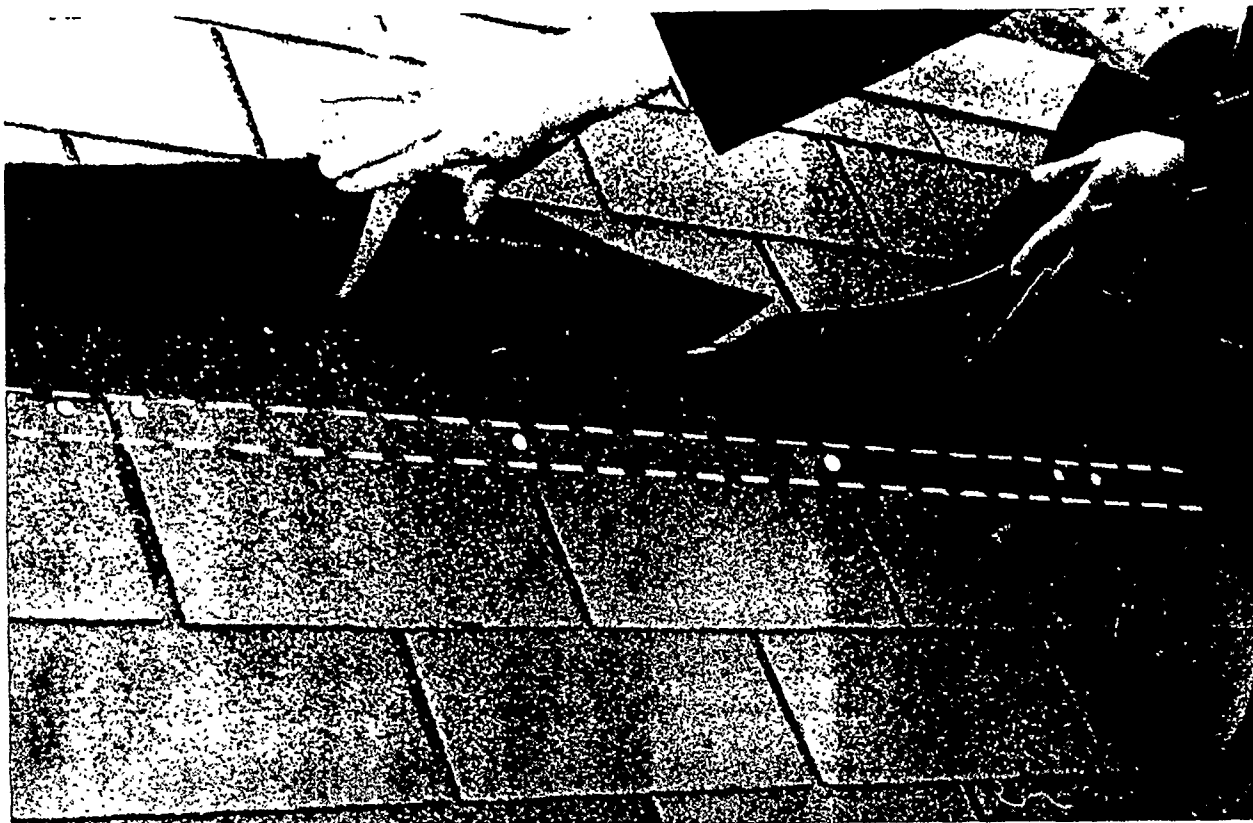
Figure 28. Proper method of nailing asphalt shingles.
