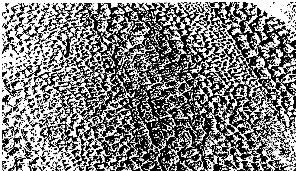
Figure 17. Alligatoring and cracking of a cold coating over alligatored asphalt surface after 1 year exposure.
