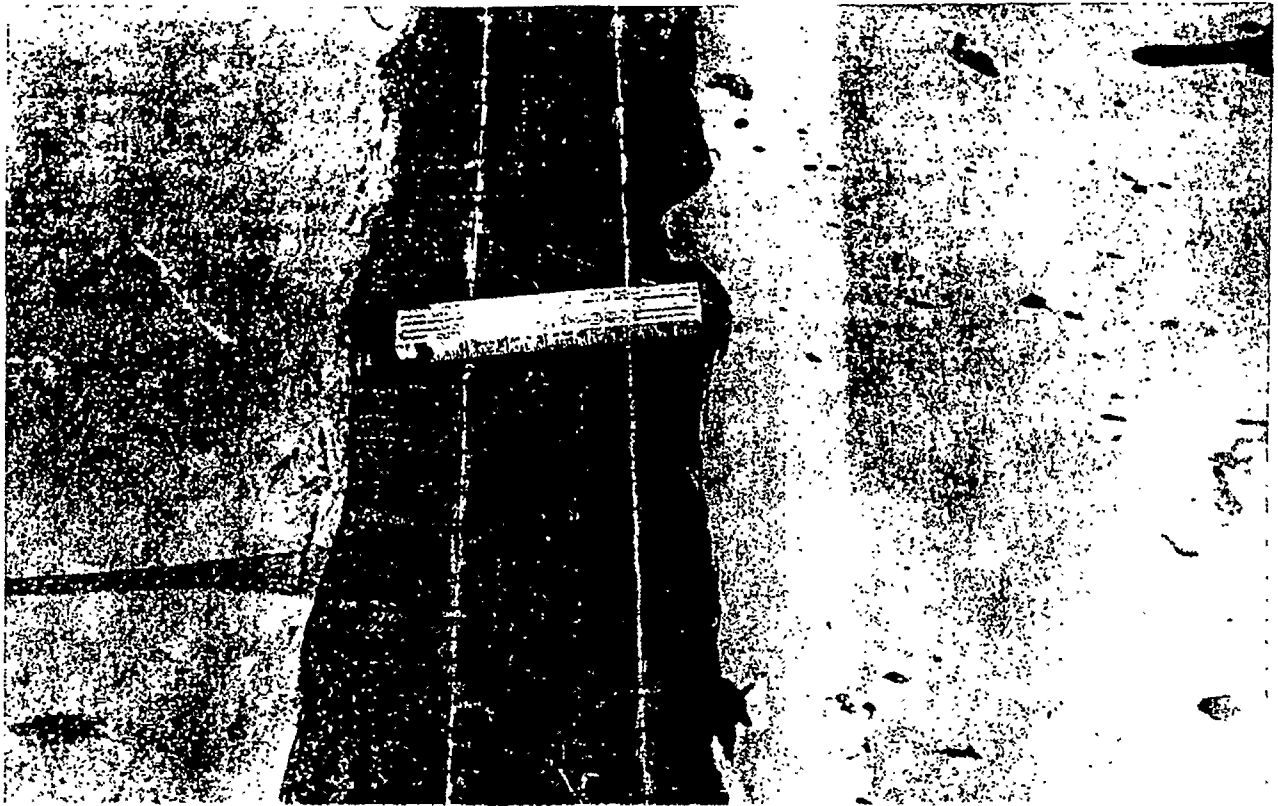
Figure 36. Closeup view—repaired roll roofing seam.
