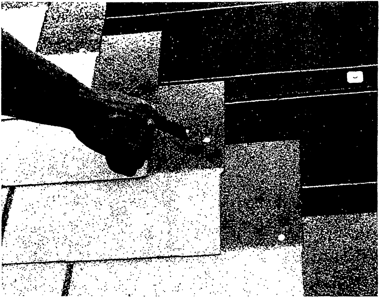
Figure 4. Asphalt shingles nailed too high.
