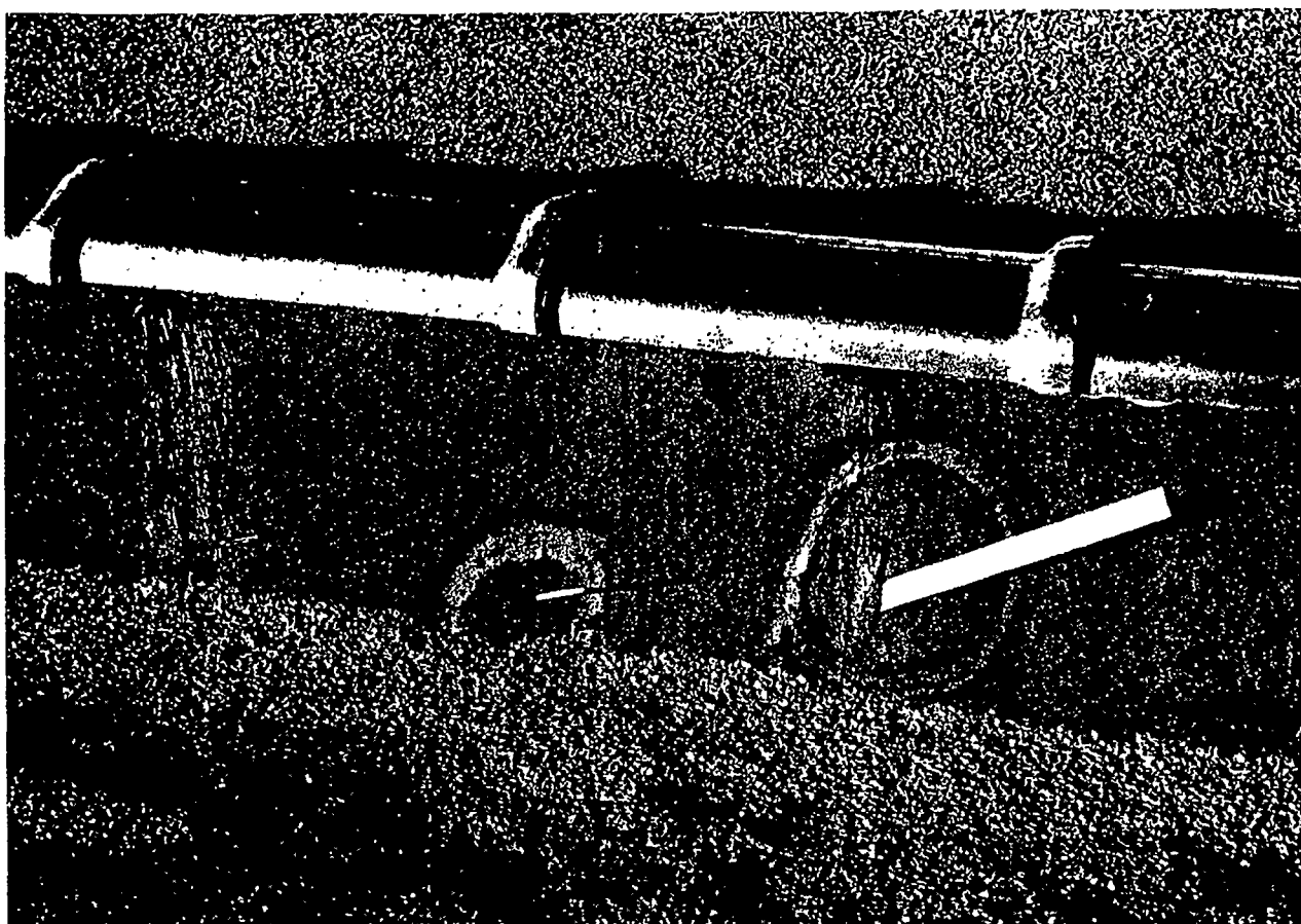
Figure 49. Open laps and split in base flashing.
