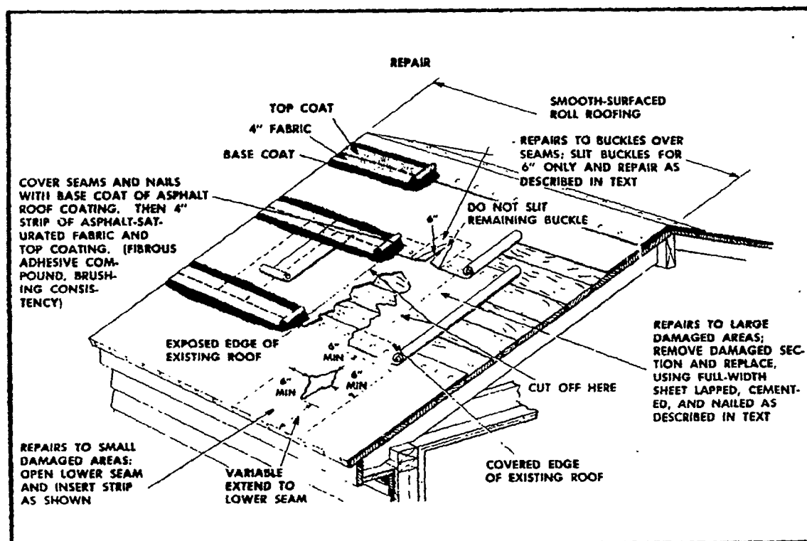
Figure 35. Repairing asphalt roll roofing.
