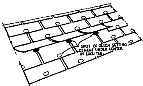
Figure 29. Location of cement under tabs.
