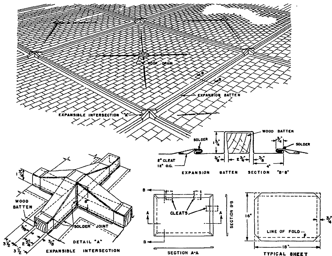
Figure 45. Flat seam roofing.
