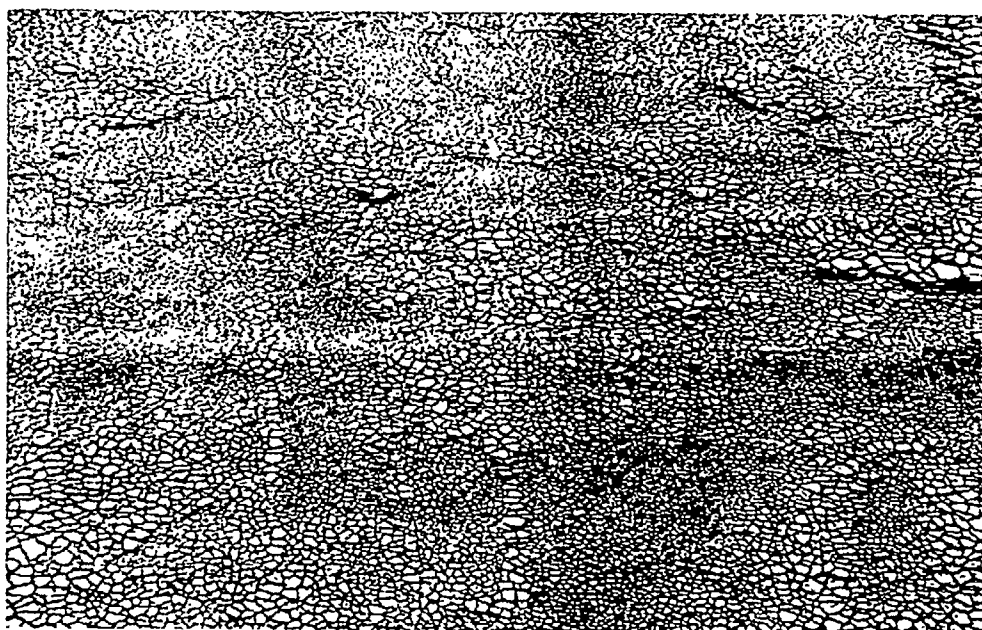
Figure 2. Alligatoring caused by heavy application of asphalt on smooth-surfaced built-up roof.
