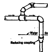
FIG. 36. DRIPPING MAIN WHERE IT RISES TO HIGHER LEVEL
