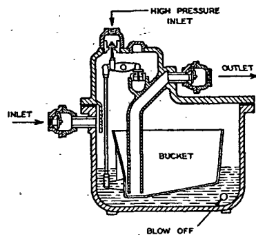
FIG. 34. LIFTING TRAP
