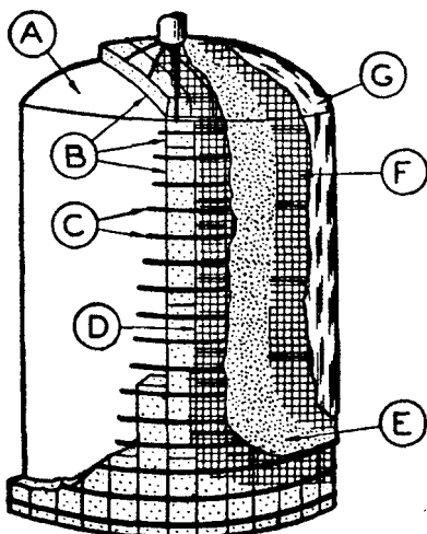
FIGURE 14. Application of mineral wool block insulation on curved surfaces.
