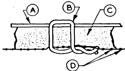
FIGURE 9. Blanket insulation held on by hairpin wires through twin holes in metal surfaces.
