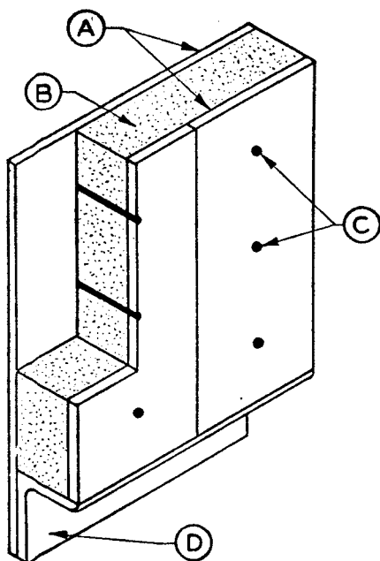
FIGURE 1. Insulation enclosed between metal sheets.
