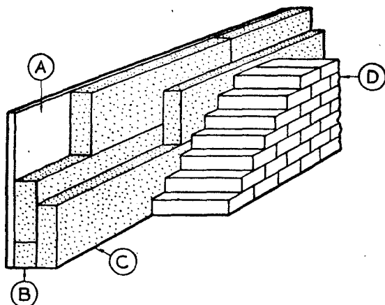
FIGURE 16. Application of mineral wool blocks between structural supports.
