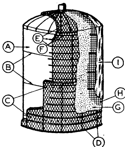
FIGURE 13. Application of mineral wool blanket insulation on curved surfaces.
