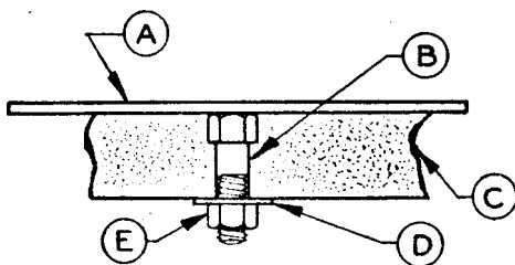
FIGURE 6. Insulation attached by bolts with heads welded to metal surface.
