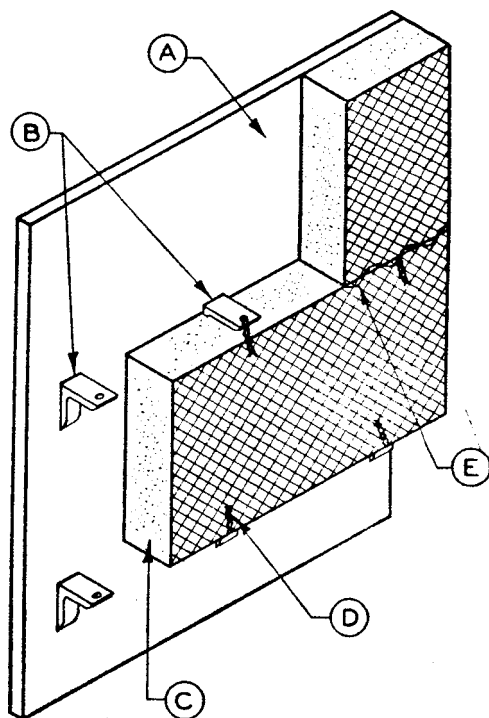
FIGURE 3. Blanket insulation supported by clip angles.
