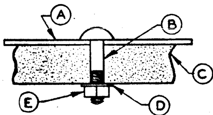
FIGURE 7. Insulation attached by bolts through drilled holes.
