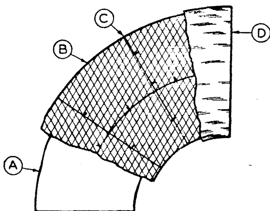
FIGURE 20. Application of blanket-type mineral wool pipe insulation on large valves and fittings.
