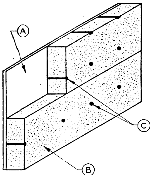
FIGURE 5. Insulation attached by welding with stud gun after insulation is in place.
