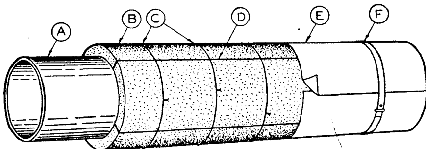
FIGURE 23. Application of mineral wool segmental pipe insulation.
