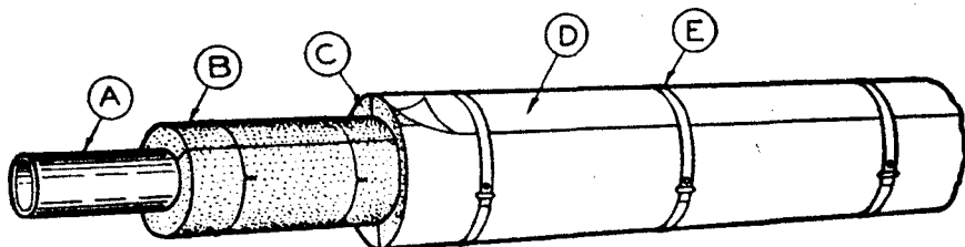
FIGURE 24. Application of mineral wool sectional pipe insulation, double-layer.
