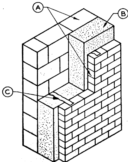
FIGURE 2. Insulation enclosed between masonry walls.
