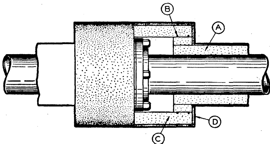
FIGURE 26. Application of molded-type mineral wool pipe insulation to flanges and fittings.
