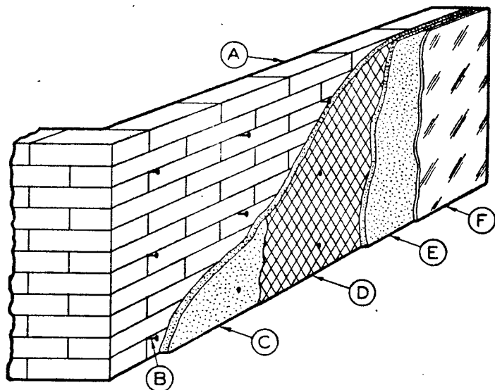
FIGURE 18. Application of mineral wool insulating cement on brick surface.
