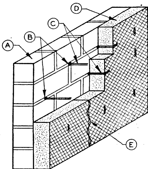
FIGURE 11. Application of blanket insulation by hairpin wires affixed to nails embedded in masonry joints.
