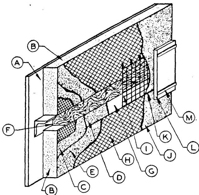
FIGURE 12. Expansion joints for large metal vessels (see par. 16d).
