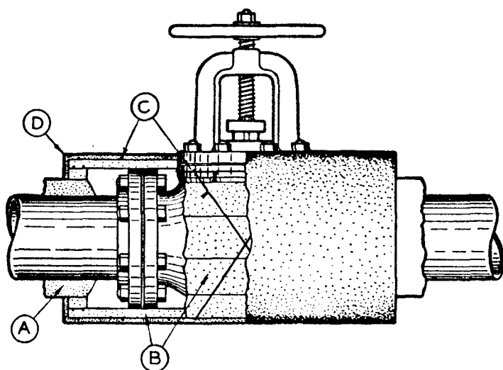
FIGURE 25. Application of mineral wool block insulation to large fittings.
