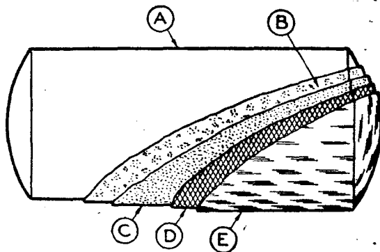
FIGURE 17. Application of mineral wool insulating cement on curved steel surfaces.
