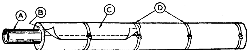
FIGURE 22. Application of mineral wool sectional pipe insulation, single-layer. A, Bare pipe; B, sectional pipe insulation; C, canvas jacket or other specified finish; D, metal bands.
