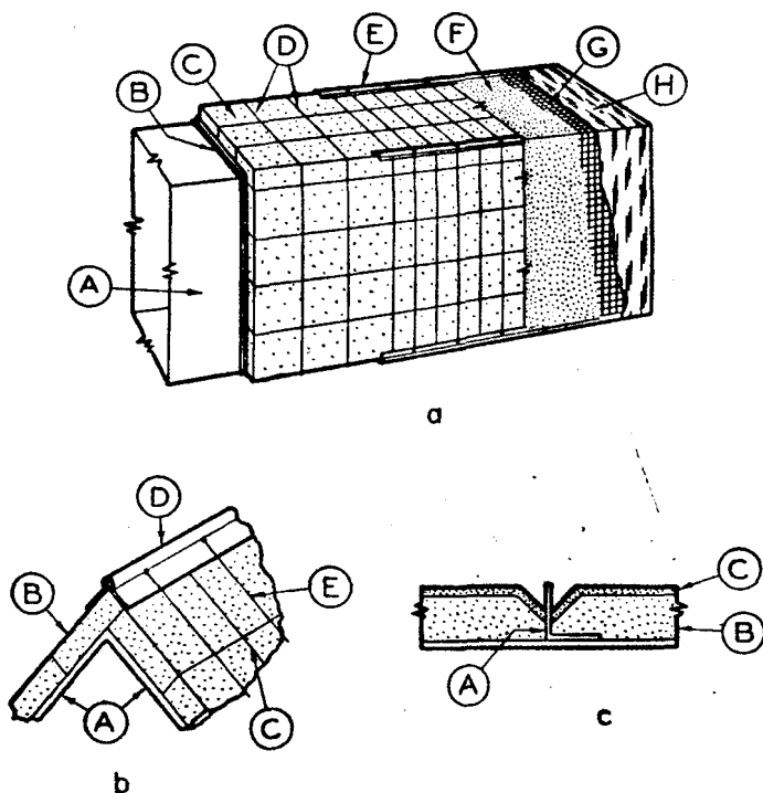
FIGURE 15. Application of mineral wool blocks on flat or rectangular surfaces.
