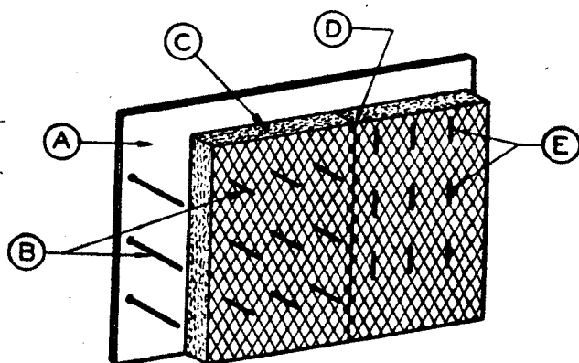
FIGURE 4. Blanket insulation impaled on wires.
