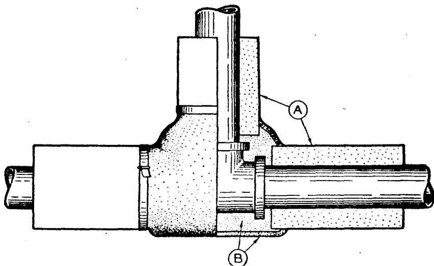
FIGURE 21. Application of mineral wool insulating cement to valves, flanges, and fittings.
