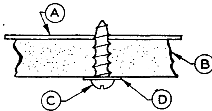
FIGURE 8. Insulation attached to light-gage metal surface by sheet metal screw and washer.
