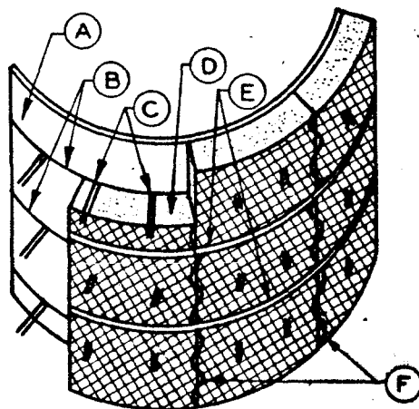
FIGURE 10. Blanket insulation held on by tie wires attached to wire girdles and exterior circumferential bands.
