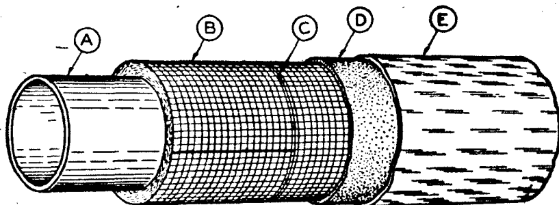
FIGURE 19. Application of blanket-type mineral wool pipe insulation on pipes.
