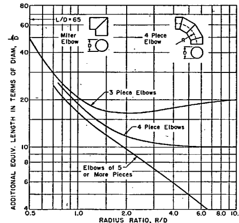
FIG. 6. LOSS IN 90-DEG ELBOWS OF ROUND CROSS-SECTION
