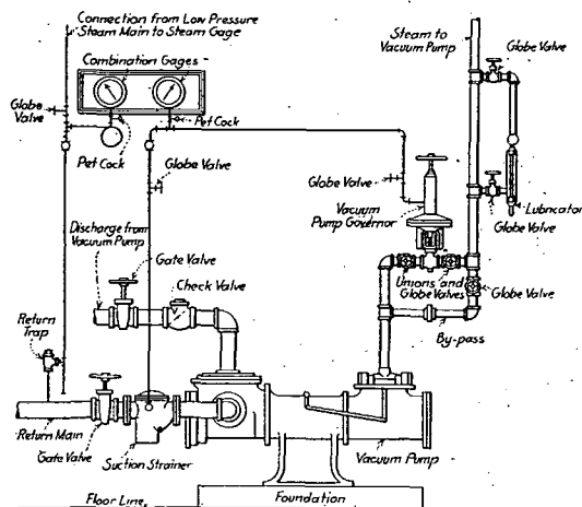
FIG. 7. METHOD OF MAKING CONNECTION TO STEAM-OPERATED VACUUM PUMP
