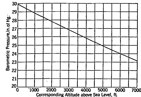
FIG. 4. RELATION BETWEEN BAROMETRIC PRESSURE AND ALTITUDE
