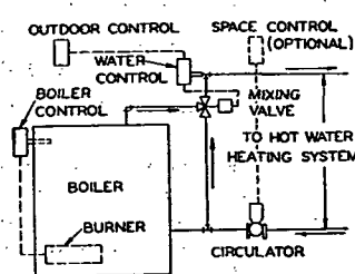
FIG. 8. CONTROL OF HOT WATER HEATING WITH PROVISIONS FOR DOMESTIC WATER HEATING (Limit and primary controls not shown)
