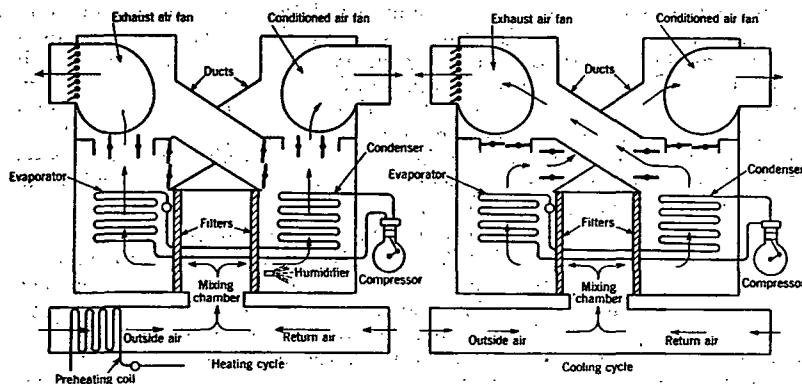
FIG. 9. SCHEMATIC OPERATION OF REVERSED CYCLE CONDITIONING SYSTEM
