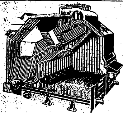
INTEGRAL FURNACE BOILER
